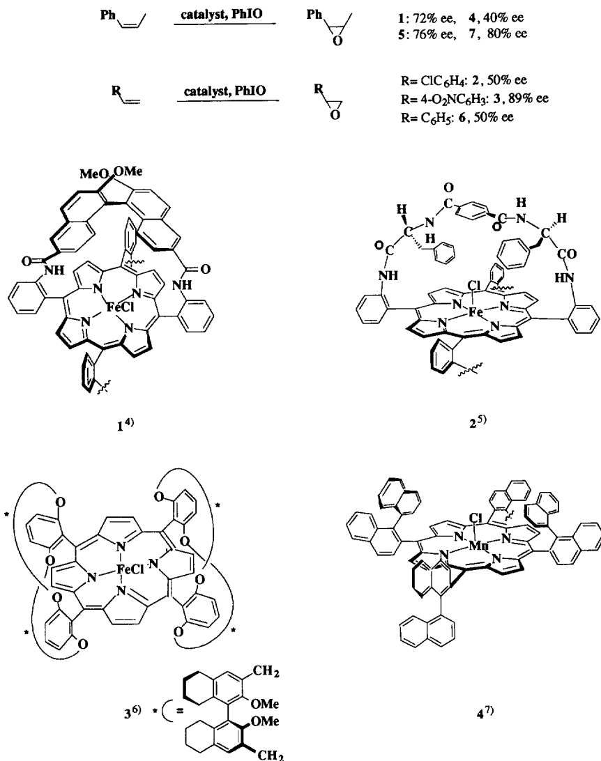
Fig. 2. Examples of porphyrin-catalysed asymmetric epoxidation.
