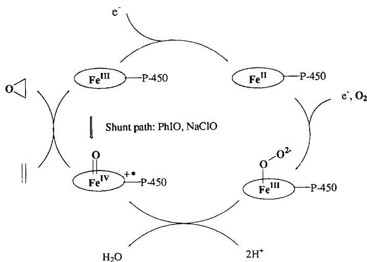
Fig. 1. Catalytic cycle of cytochrome P-450.
