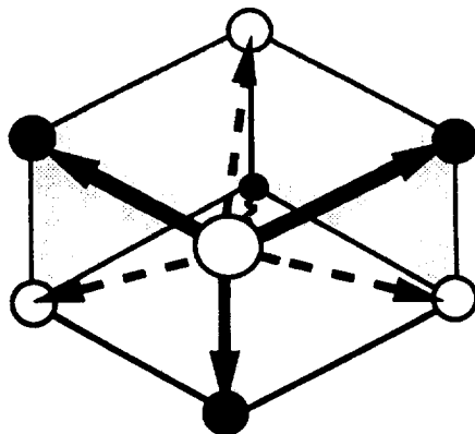
Fig. 2. The \mathcal{S}_8^{\downarrow\mathcal{C}} automorphism associated with a \{3J, 3J', 3J''\} interaction set. Reproduced with permission from Ref.[9].
