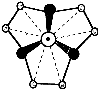
Fig. 4. The \mathcal{S}_{20} \uparrow \mathcal{A}_5 automorphism associated with a \{3J, 6J', (3J'', 6J'''), J''''\} interaction set, in a contracted view of \mathcal{S}_{20} \uparrow \mathcal{A}_5 spin symmetry subduced further to C_3 at the spin site chosen. The subset components in parentheses are omitted for clarity.
