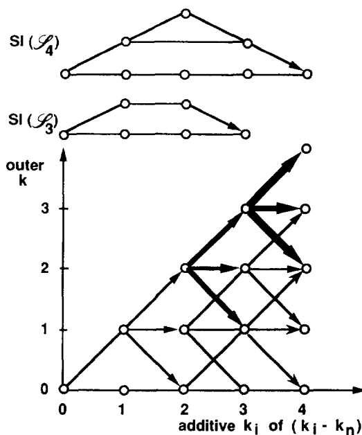
Fig. 8. Propagative k_i - k_n recoupling over Liouville space of the 2 \leq n \leq 4, \dots -fold spin 1/2 cluster. The diagram, after Ref. [69a], gives the pictorial forms for two scalar invariants. In addition, it incorporates a small correction to the original version.
