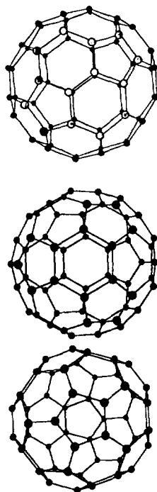
Fig. 6. Diagram showing the \mathcal{J}_h structure of \text{C}_{60} fullerene as viewed along the C_2 , C_3 and C_5 axes; note the separation between the 5-membered ring components of the structure. The symmetry axes are centred about mid-edge or face centre of the cage solid. (From Ref. [18] with permission.)
