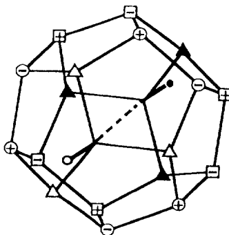
Fig. 5. A mathematical model for \{\chi_i\} of the module and scalar invariant :3^611: ( SU8 \times \mathcal{S}_{20}^1 \mathcal{A}_5 ) as a determinable invariance set. One further analogous projective geometry derived from a higher regular solid is known [49]. Reproduced with permission from Ref.[49a].
