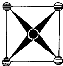
Fig. 1. The \mathcal{S}_6^{\downarrow\mathcal{C}} automorphism associated with a \{4J, J'\} interaction set.
