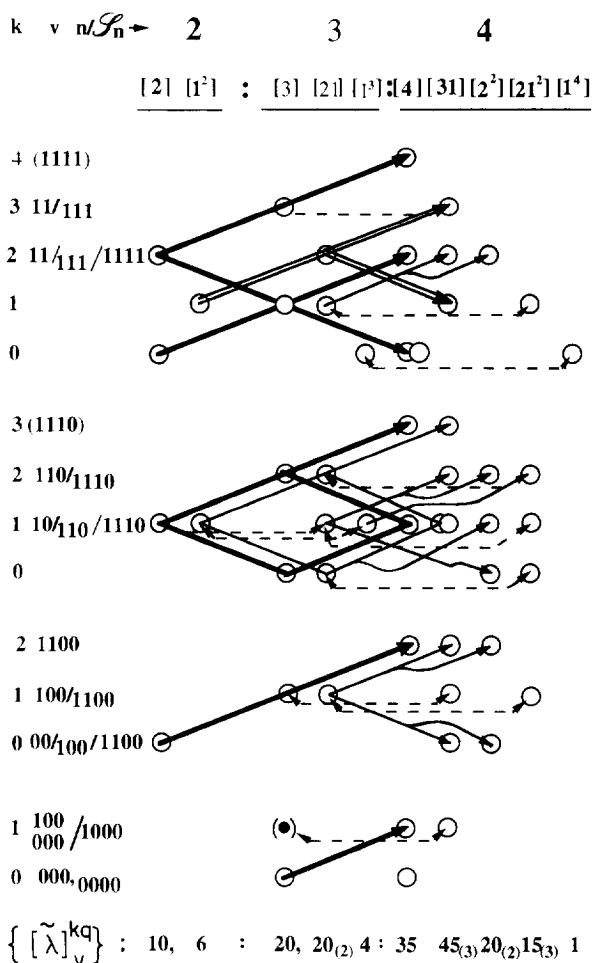
Fig. 9. A view of propagation and branching over specific \tilde{H}_i carrier subspatial sets associated with SU2 \times \mathcal{S}_n Liouville spin space of [A]_n clusters, from Ref. [69a] with permission; here v arises from recoupling which under democratic recoupling becomes associated with \mathcal{S}_n -induced symmetry.
