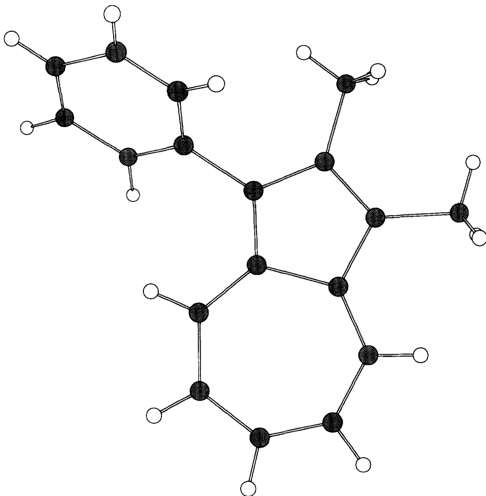
Fig. 11. The structure of 1-phenyl-2,3-dimethylazulene.
