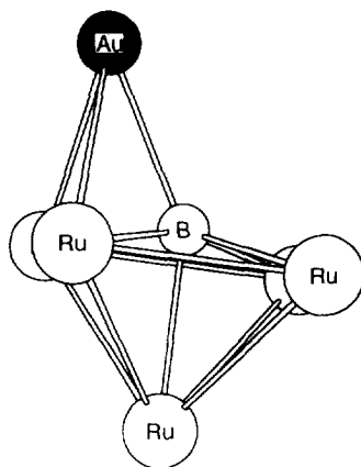
Fig. 19. The \{\text{Ru}_5\text{BAu}\} core of [\text{Ru}_5(\text{CO})_{15}\text{B}\{\text{AuPPh}_3\}] .
