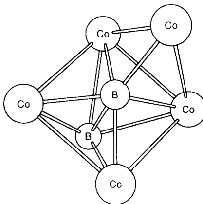
Fig. 21. The \{\text{Co}_5\text{B}_2\} core of [\text{Co}_5(\text{CO})_{14}\text{B}(\text{BH})] .
