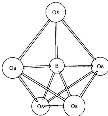
Fig. 20. The \{\text{Os}_5\text{B}\} core of [\text{HOs}_5(\text{CO})_{16}\text{B}] .
