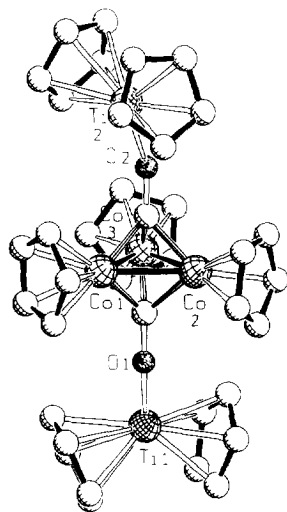
Fig. 8. Molecular structure of [(\text{CpCo})_3(\text{COTiCp}_2)_2] 51 .
