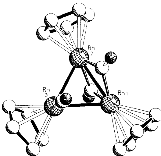
Fig. 4. Molecular structure of C_s -[(CpRh) _3 (CO) _3 ] 11B .
