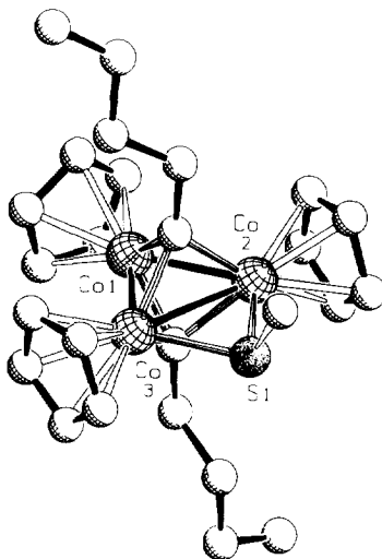
Fig. 28. Molecular structure of [(\text{CpCo})_3(\text{C}^i\text{Bu})_2(\text{SMe})]^+ 117 .
