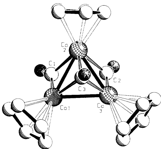
Fig. 2. Molecular structure of [(\text{CpCo})_3(\text{CO})_3] 8a .
