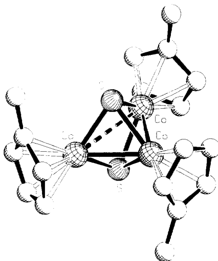
Fig. 16. Molecular structure of [(\text{Cp}'\text{Co})_3\text{S}_2] 60b .
