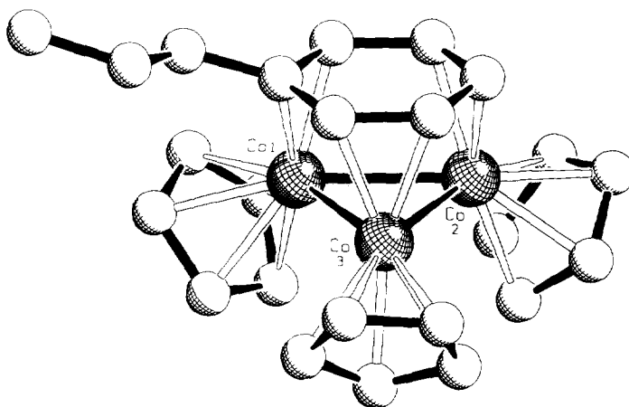
Fig. 34. Molecular structure of [(CpCo) 3 (β-methylstyrene)] 98a .
