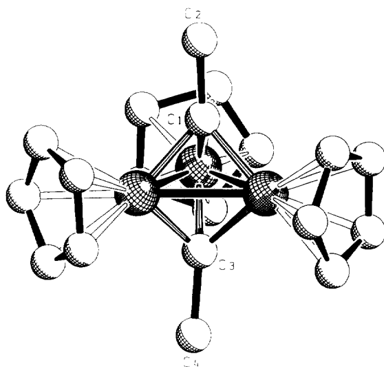
Fig. 25. Molecular structure of [(\text{CpCo})_3(\text{CMe})_2] 88i .
