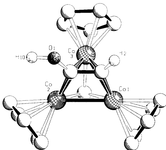
Fig. 21. Molecular structure of [(\text{CpCo})_3(\text{CH})(\text{HCCOH})]^+ 93 .
