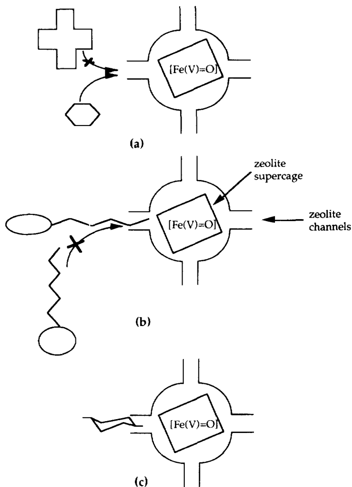
Fig. 17. Schematic representation of (a) substrate, (b) regio- and (c) stereoselectivities in zeolite cages containing the [\text{Fe}(\text{V})=\text{O}]^+ oxo species (adapted from Ref. [8]).
