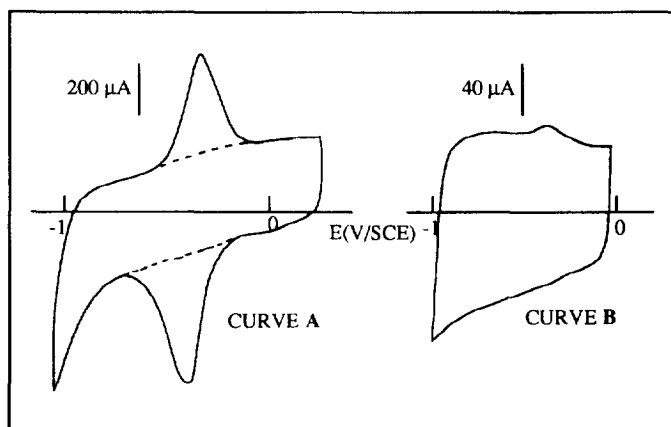
Fig. 16. Cyclic voltammogram of a pressed graphite powder-composite electrode containing (curve A) Y-zeolite-encapsulated Fe III Salen and (curve B) Y-zeolite surface-adsorbed Fe III Salen in DMSO + 0.1 M LiClO 4 solution (potential sweep rate = 10 mV s -1 ) (adapted from Refs. [98,101]).
