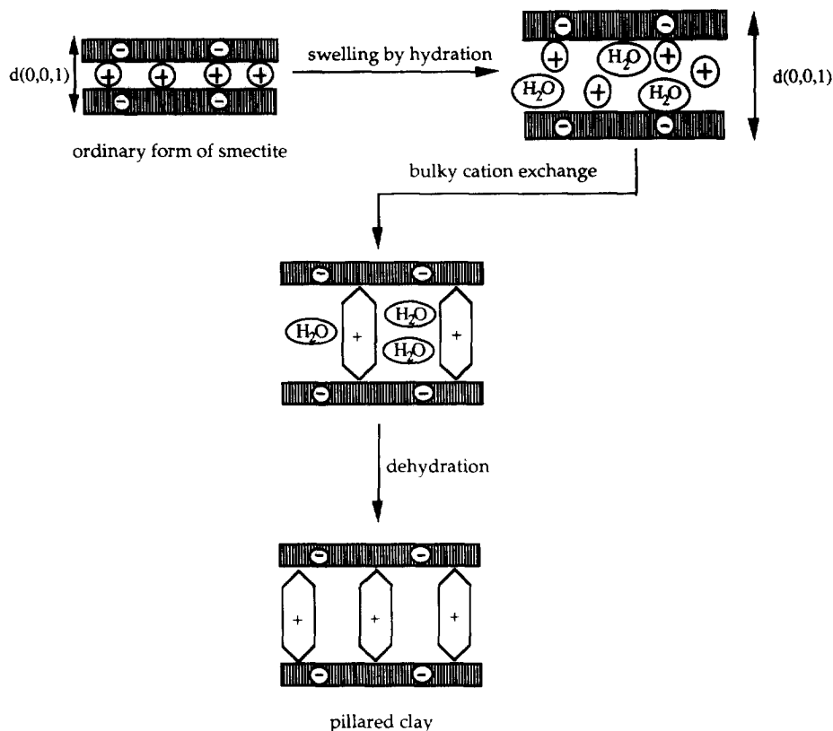
Fig. 5. General scheme for the synthesis of pillared clays (adapted from Ref. [18]).
