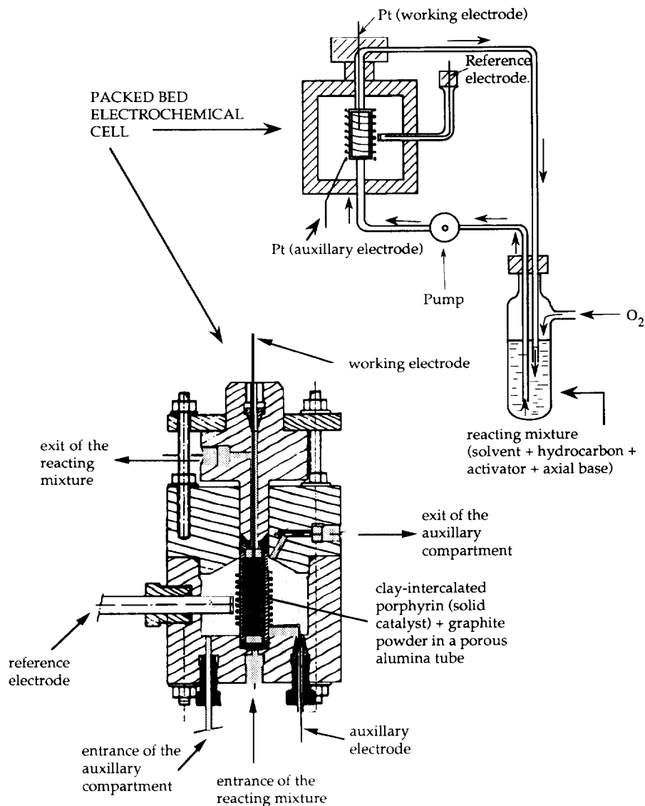
Fig. 11. Schematic illustration of the packed-bed electrochemical cell (adapted from Ref. [52]).
