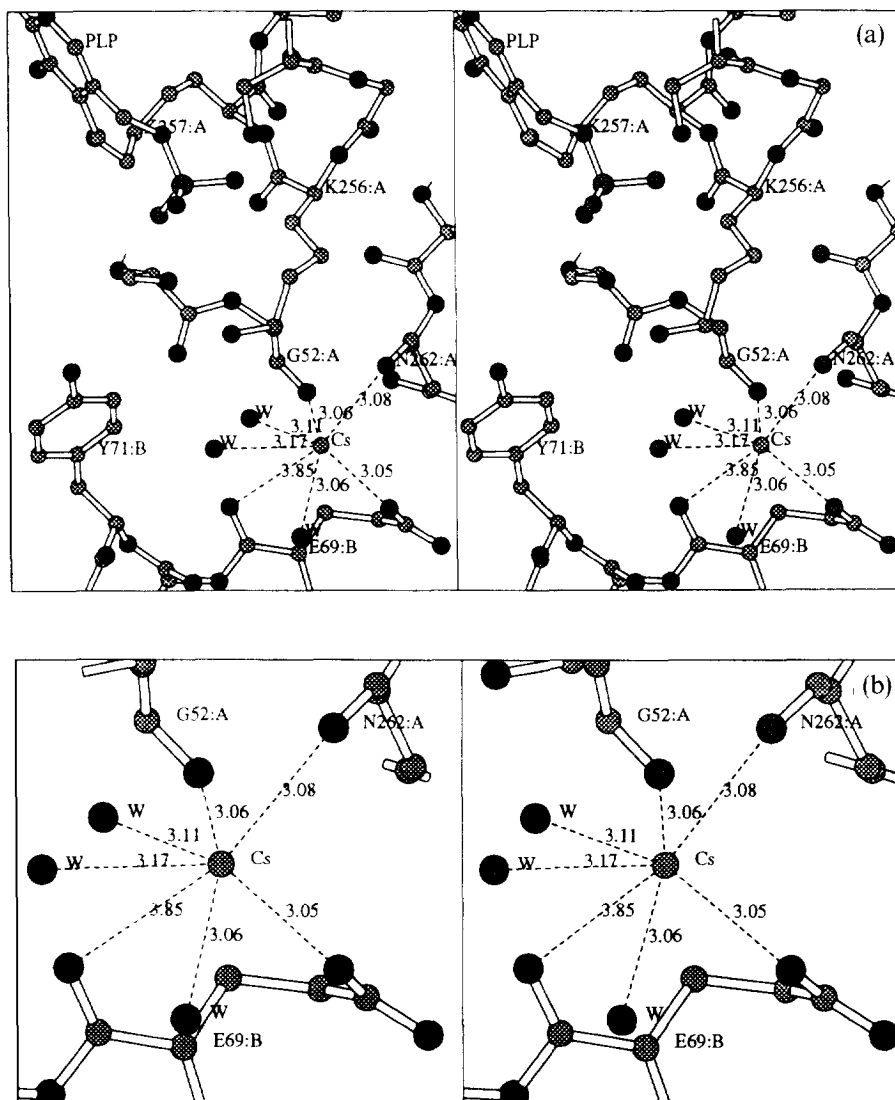
Fig. 11. Stereo drawings of the X-ray structure of Cs + bound to the K + site of TPL. (a) Details of the Cs + complex showing the relationship of the metal ion site to the active site. PLP (upper left-hand corner) is separated from the metal site by Lys256 from subunit A and by Tyr71 from subunit B. (b) Close-up view of the bonding to Cs + . (Drawing provided courtesy of A.A. Antson.)
