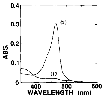
Fig. 16. UV-Visible quasi-static absorbance spectra of the quinonoid formed in the reaction of 6\ \mu\text{M} \alpha_2\beta_2 with 40\ \text{mM} L-Ser and 2\ \text{mM} indoline (an indole analogue [138]) in the absence (curve (1)) and in the presence (curve (2)) of 100\ \text{mM} \text{Na}^+ .
