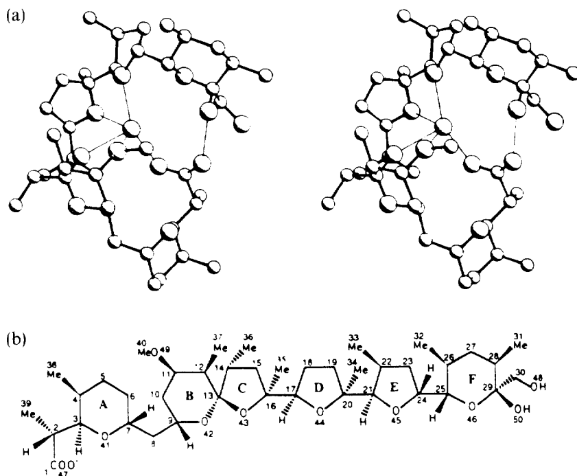
Fig. 5. (a) Stereo drawing of the X-ray structure of the nigericin·Ag + complex. (Taken from Ref. [81] with permission.) (b) Schematic diagram of uncomplexed nigericin. (Taken from Ref. [89] with permission.)
