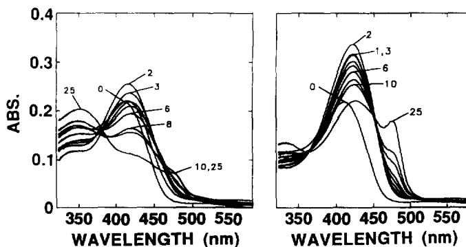
Fig. 17. RSSF spectra for the reaction of \alpha_2\beta_2 with L-Ser and IGP (the \alpha\beta reaction; see Eq. (11) and Scheme 3) in the absence (left) and in the presence (right) of 100 mM \text{Na}^+ (concentrations: [\alpha_2\beta_2] = 18 \mu\text{M} ; [\text{L-Ser}] = 40 \text{ mM} ; [\text{IGP}] = 0.5 \text{ mM} ). The numbered spectra are taken at the following time points after flow stopped: spectrum 0, 0 s; spectrum 2, 0.017 s; spectrum 3, 0.026 s; spectrum 4, 0.034 s; spectrum 5, 0.043 s; spectrum 6, 0.06 s; spectrum 8, 0.094 s; spectrum 10, 0.128 s; spectrum 25, 1.709 s.
