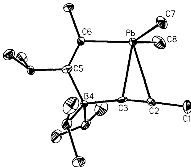
Fig. 4. Molecular structure of the zwitterionic intermediate obtained from the 1,1'-organoboration reaction between ^1\text{Pr}_3\text{B} and \text{Me}_2\text{Pb}(\text{C}\equiv\text{CMe})_2 [78]. Selected bond lengths (picometres) and bond angles (degrees) are as follows: \text{Pb}-\text{C}(2) , 264.8(8); \text{Pb}-\text{C}(3) , 246.7(6); \text{Pb}-\text{C}(6) , 220.3(6); \text{Pb}-\text{C}(7) , 222.2(7); \text{Pb}-\text{C}(8) , 220.2(7); \text{B}-\text{C}(3) , 164.0; \text{B}-\text{C}(5) , 164.8(8); \text{C}(5)-\text{C}(6) , 133.4(9); \text{C}(2)-\text{C}(3) , 121.0(10); \text{BC}(3)\text{C}(2) , 169.5(6); \text{C}(1)\text{C}(2)\text{C}(3) , 177.3(7).
