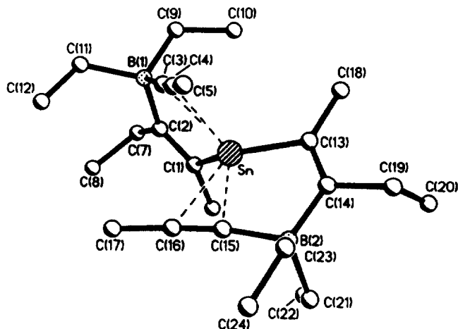
Fig. 9. Molecular structure of the zwitterionic intermediate 58 obtained from the 1,1-organoboration reaction between two equivalents of \text{Et}_3\text{B} and one equivalent of \text{Sn}(\text{C}\equiv\text{CMe})_4 [74]. Selected bond lengths (picometres) and bond angles (degrees) are as follows: \text{Sn}-\text{C}(3) , 235.5(3); \text{Sn}-\text{C}(4) , 251.1(3); \text{Sn}-\text{C}(1) , 211.7(3); \text{Sn}-\text{C}(13) , 212.2(3); \text{Sn}-\text{C}(15) , 235.1(3); \text{Sn}-\text{C}(16) , 253.5(3); \text{B}(1)-\text{C}(3) , 164.3(5); \text{B}(1)-\text{C}(2) , 163.4(5); \text{C}(1)-\text{C}(2) , 133.7(4); \text{C}(3)-\text{C}(4) , 122.7(5); \text{C}(1)\text{SnC}(13) , 140.9(1); \text{B}(1)\text{C}(3)\text{C}(4) , 172.7(3); \text{C}(3)\text{C}(4)\text{C}(5) , 175.8(3).
