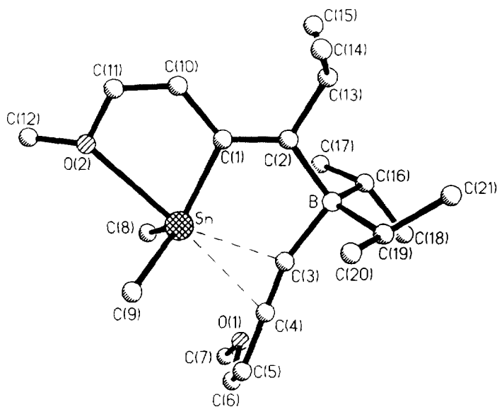
Fig. 8. Molecular structure of the zwitterionic intermediate obtained from the 1,1-organoboration reaction between ^1\text{Pr}_3\text{B} and \text{Me}_2\text{Sn}(\text{C}\equiv\text{C}-\text{CH}=\text{CH}-\text{OMe})_2 [68]. Selected bond lengths (picometres) and bond angles (degrees) are as follows: \text{Sn}-\text{C}(3) , 237.3(3); \text{Sn}-\text{C}(4) , 266.1(3); \text{Sn}-\text{C}(1) , 212.7(3); \text{Sn}-\text{C}(8) , 211.3(5); \text{Sn}-\text{C}(9) , 211.5(5); \text{Sn}-\text{O}(2) , 259.2; \text{B}-\text{C}(3) , 165.0(5); \text{B}-\text{C}(2) , 164.3(4); \text{C}(1)-\text{C}(2) , 135.3(4); \text{C}(3)-\text{C}(4) , 122.1(5); \text{BC}(3)\text{C}(4) , 163.5(3); \text{C}(3)\text{C}(4)\text{C}(5) , 179.2(4).
