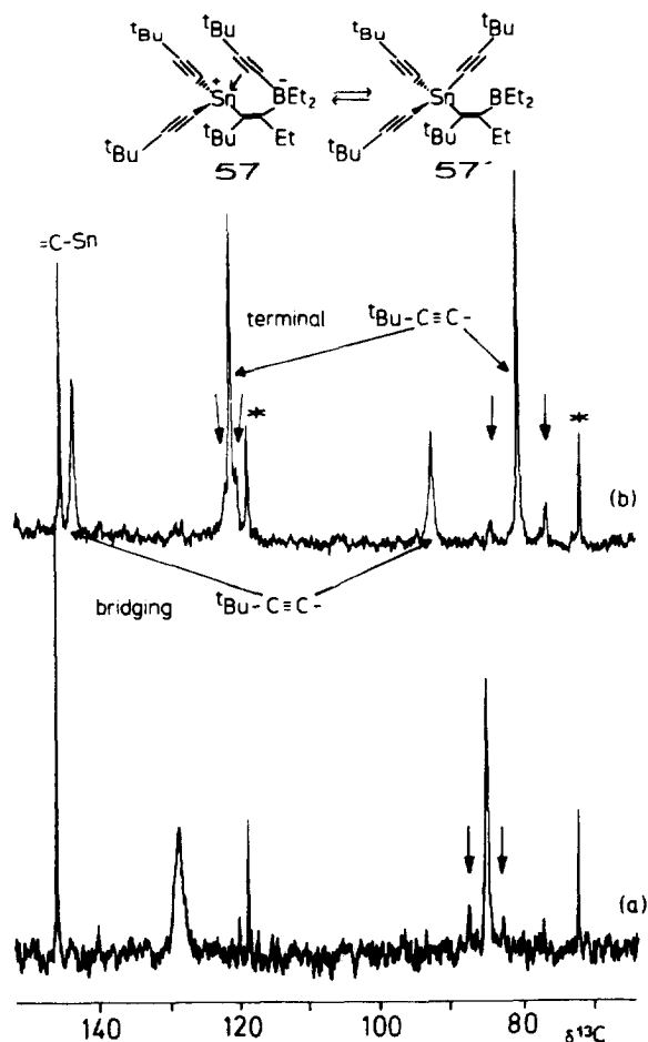
Fig. 2. 75.5 MHz ^{13}\text{C}(^1\text{H}) NMR spectra at various temperatures in \text{CD}_2\text{Cl}_2 , demonstrating the dynamic behaviour of the zwitterionic intermediate 57 ( \text{R}^1 = ^t\text{Bu} , \text{R} = \text{Et} ); ^{117}/^{119}\text{Sn} satellites are marked by arrows; the ^{13}\text{C}(\text{C}\equiv\text{C}) resonances belonging to a small amount of the starting material \text{Sn}(\text{C}\equiv\text{C}^t\text{Bu})_4 are marked by asterisks. (a) At -30^\circ\text{C} ; there is rapid exchange between terminal and bridging alkynyl groups. (b) At -75^\circ\text{C} ; the ^{13}\text{C} NMR signals for the alkynyl groups are now split in those for terminal and bridging groups as indicated.
