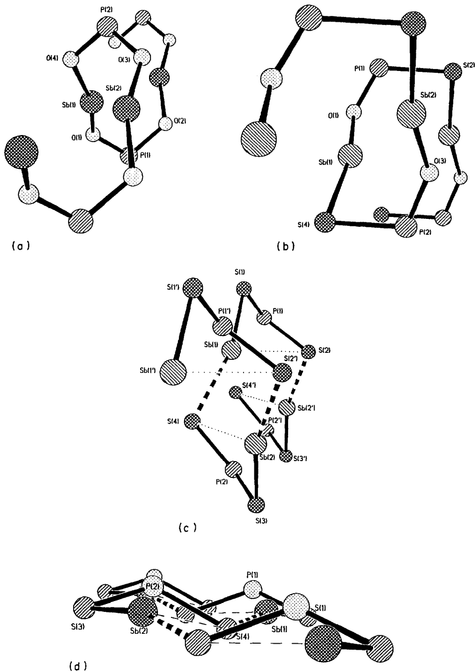
Fig. 10. View of the polymeric catena down the polymer axis in (a) [\text{Ph}_2\text{SbO}_2\text{PPh}_2]_n , (b) [\text{Ph}_2\text{SbOSPPH}_2]_n , (c) [\text{Ph}_2\text{SbS}_2\text{P}(\text{OPr}^t)_2]_n , and (d) [\text{Me}_2\text{SbS}_2\text{PMe}_2]_n .
