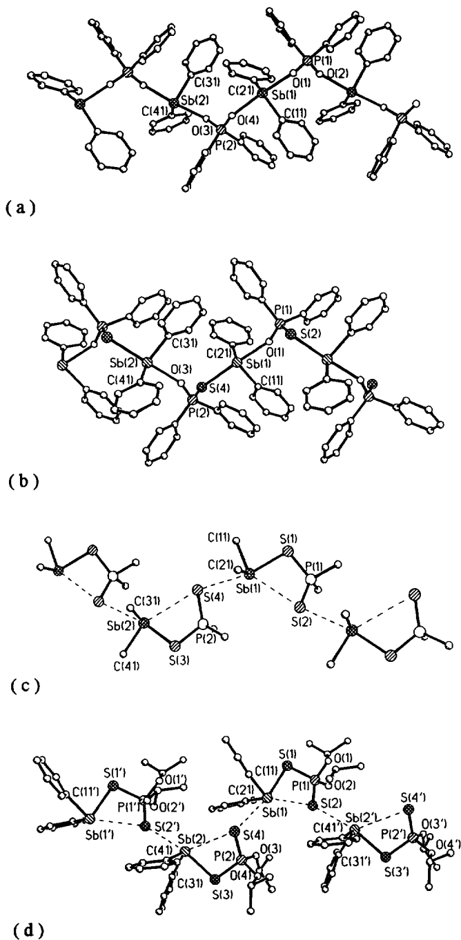
Fig. 9. View of the polymeric association in (a) [\text{Ph}_2\text{SbO}_2\text{PPh}_2]_n , (b) [\text{Ph}_2\text{SbOSPPH}_2]_n , (c) [\text{Me}_2\text{SbS}_2\text{PMe}_2]_n , and (d) [\text{Ph}_2\text{SbS}_2\text{P}(\text{OPr}^i)_2]_n .
