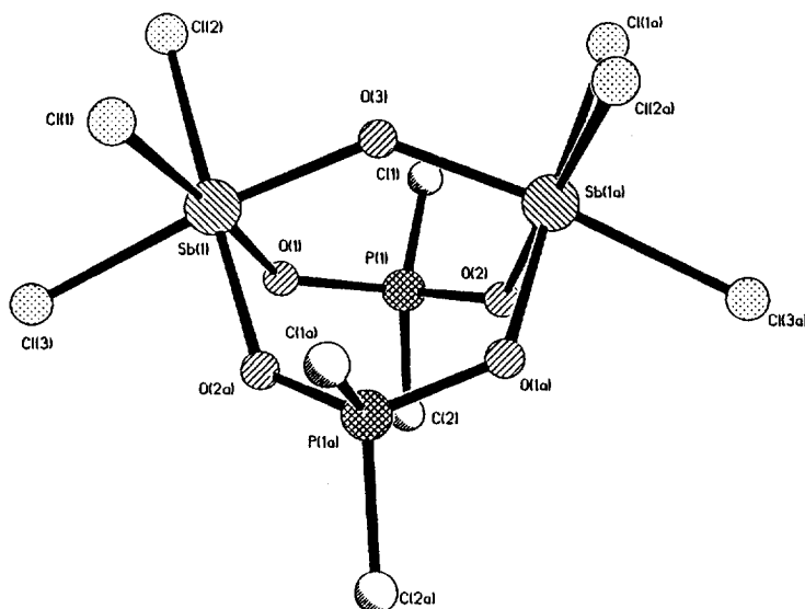
Fig. 11. The molecular structure of [\text{Cl}_3\text{Sb}(\text{O}_2\text{PMe}_2)]_2\text{O} .
