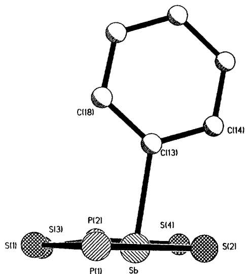
Fig. 6. The phenyl ring orientation in \text{PhSb}[\text{S}_2\text{P}(\text{OPr}^i)_2]_2 .
