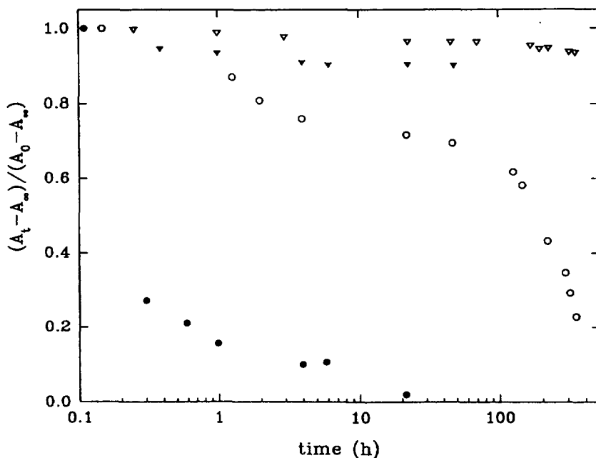
Fig. 4. Spectrophotometric evidences for \text{Al}(\text{acac})_3 and of \text{Al}(\text{malt})_3 (meta)stability in water at \text{pH} \approx 7 at 25^\circ\text{C} . A_0 , A_t and A_\infty indicate the optical density at t=0 , t and after complete hydrolysis at 340 nm, for \text{Al}(\text{acac})_3 10^{-4} M (○) and 5 \times 10^{-5} M (●), and at 280 nm for \text{Al}(\text{malt})_3 10^{-4} M (▽) and 5 \times 10^{-5} M (▼) (cell path = 1 cm).
