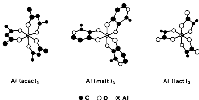
Fig. 2. Molecular structures of \text{Al}(\text{III}) synthetic toxins. Hydrogen atoms are omitted. For hydrolytic stability and lipophilicity, see Ref. [9]. (From Ref. [9], with permission.)
