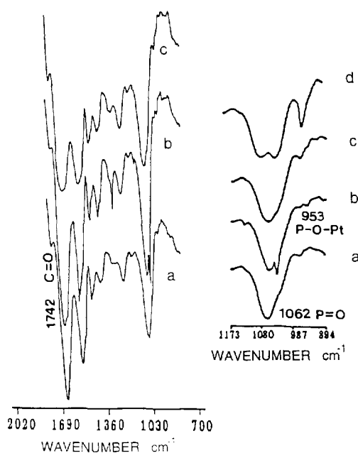
Fig. 1. IR spectra of human erythrocyte membrane ( 2\text{ mg protein ml}^{-1} ) in the presence of cis -DCDP ( 1\text{ mmol l}^{-1} ) and trans -DCDP ( 1\text{ mmol l}^{-1} ) after incubation ( 4^\circ\text{C} ) with cis -DCDP for 0 h (spectra a), 2.5 h (spectra b) and 12 h (spectra c) and with trans -DCDP for 0.5 h (spectrum d).
