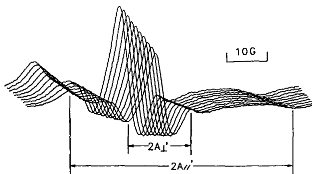
Fig. 5. Three-dimensional ESR spectra of 5DS spin labelled human erythrocyte membrane ( 2 \text{ mg protein ml}^{-1} ) as a function of the time after adding ascorbate ( 10 \text{ mmol l}^{-1} ). The time interval was 2 min and the step change of center magnetic field was 1 G automatically. 2A_{\parallel}' and 2A_{\perp}' are the parallel and perpendicular parts of the hyperfine splitting in the spectra.
