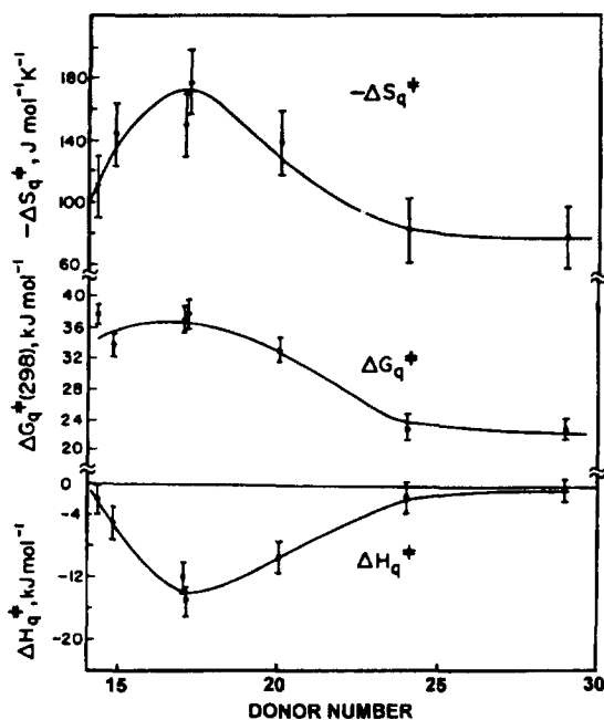
Fig. 11. Activation parameters as a function of donor number in methylene chloride. The curved lines draw through the \Delta H_q^\ddagger , \Delta S_q^\ddagger , and \Delta G_q^\ddagger (298 K) data are simply visual aids. (Reproduced with permission from Ref. [37].)
