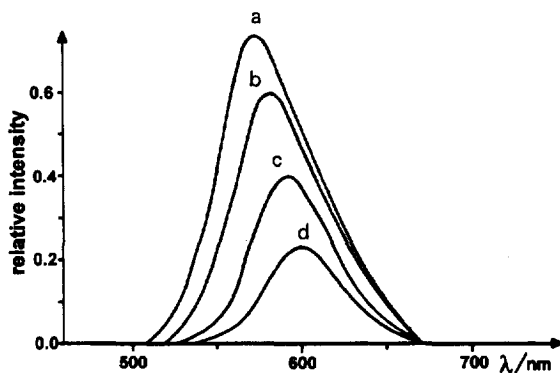
Fig. 2. Emission spectra of 1.5 \times 10^{-4} \text{ M} \text{Re}(4,7\text{-diphenyl-1,10-phenanthroline}) (\text{CO})_3\text{Cl} in decaline in the presence of (a) 0 \text{ M} , (b) 8 \times 10^{-4} \text{ M} , (c) 2 \times 10^{-3} \text{ M} and (d) 8 \times 10^{-3} \text{ M} N,N -dimethylaniline. (Reproduced with permission from Ref. [17].)
