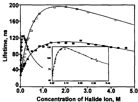
Fig. 13. Dependence of the luminescence lifetime on the concentration of halide ion in aqueous solutions of \text{Cu(CN)}_2 + \text{X}^- at 5 M ionic strength: ■ X = Cl; □ X = Br, ★ X = I. (Reproduced with permission from Ref. [40].)
