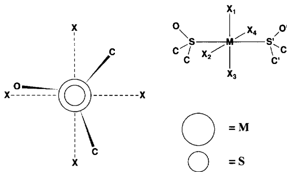
Fig. 14. Scheme of the octahedral complexes without cis S-coordinated sulfoxide. The absolute values of the torsional angle X–M–S–O are considered to describe the stereochemistry of S-coordination. The O–S–S'–O' torsional angle is considered to describe the possible reciprocal influence of two trans sulfoxides.
