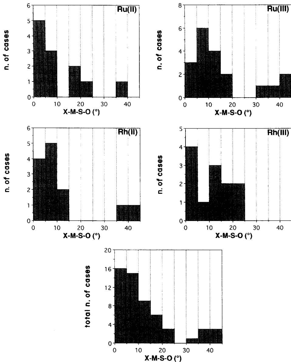
Fig. 15. Distribution of the X-M-S-O torsional angles, as defined in Fig. 14, in the cases of Ru(II), Ru(III), Rh(II), Rh(III), and all complexes.
