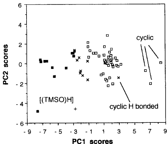
Fig. 1. Principal component analysis of the uncoordinated sulfoxides. PC2 versus PC1 scores for the free ( \square ), hydrogen bonded ( \times ) and protonated ( \blacksquare ) sulfoxides.
