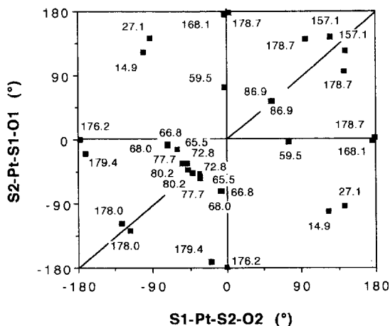
Fig.13. Dependence of the O1–S1–S2–O2 torsional angle upon S1–Pt–S2–O2 and S2–Pt–S1–O1. For sake of clarity only absolute values are reported for each point.
