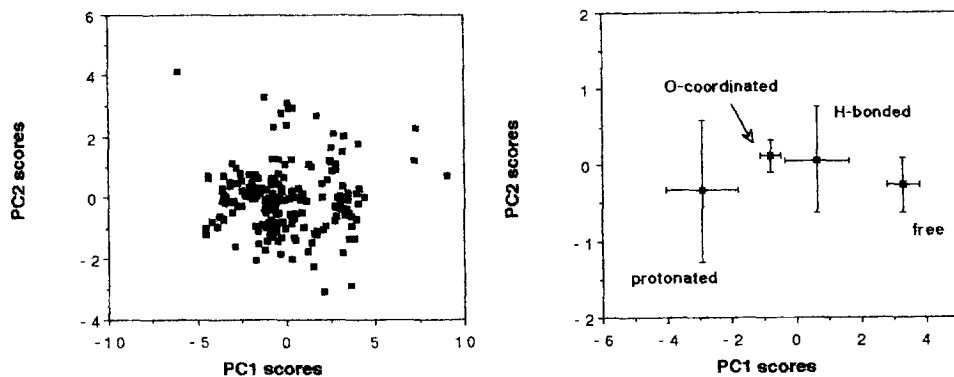
Fig. 18. Principal component analysis of coordinated sulfoxides (without S-coordinated). Interdependence of the PC1 and PC2 scores. On the right side, the mean values of the PC1 and PC2 scores, and the triple of their standard deviations, are considered for the four classes of “free”, “H-bonded”, “protonated”, and “O-coordinated” sulfoxides.
