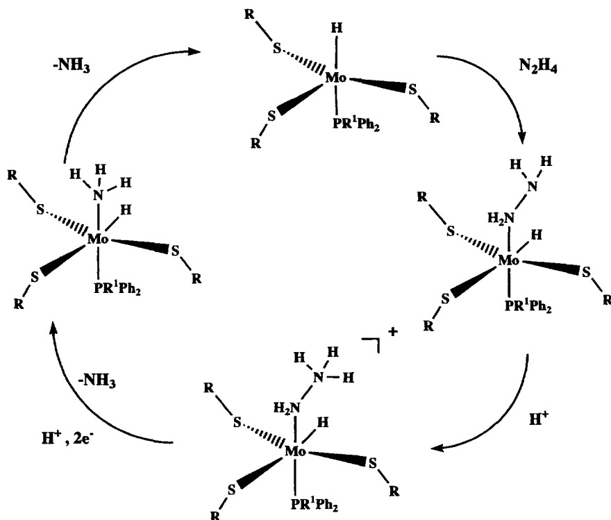
Fig. 10. Scheme of reduction of hydrazine by the complexes [\text{MoH}(\text{SR})_3(\text{PR}^1\text{Ph}_2)] ( \text{R} = \text{C}_6\text{H}_2\text{Me}_3\text{-2,4,6} or \text{C}_6\text{H}_2\text{Pr}_3\text{-2,4,6} ; \text{R}^1 = \text{Me} or \text{Et} ).
