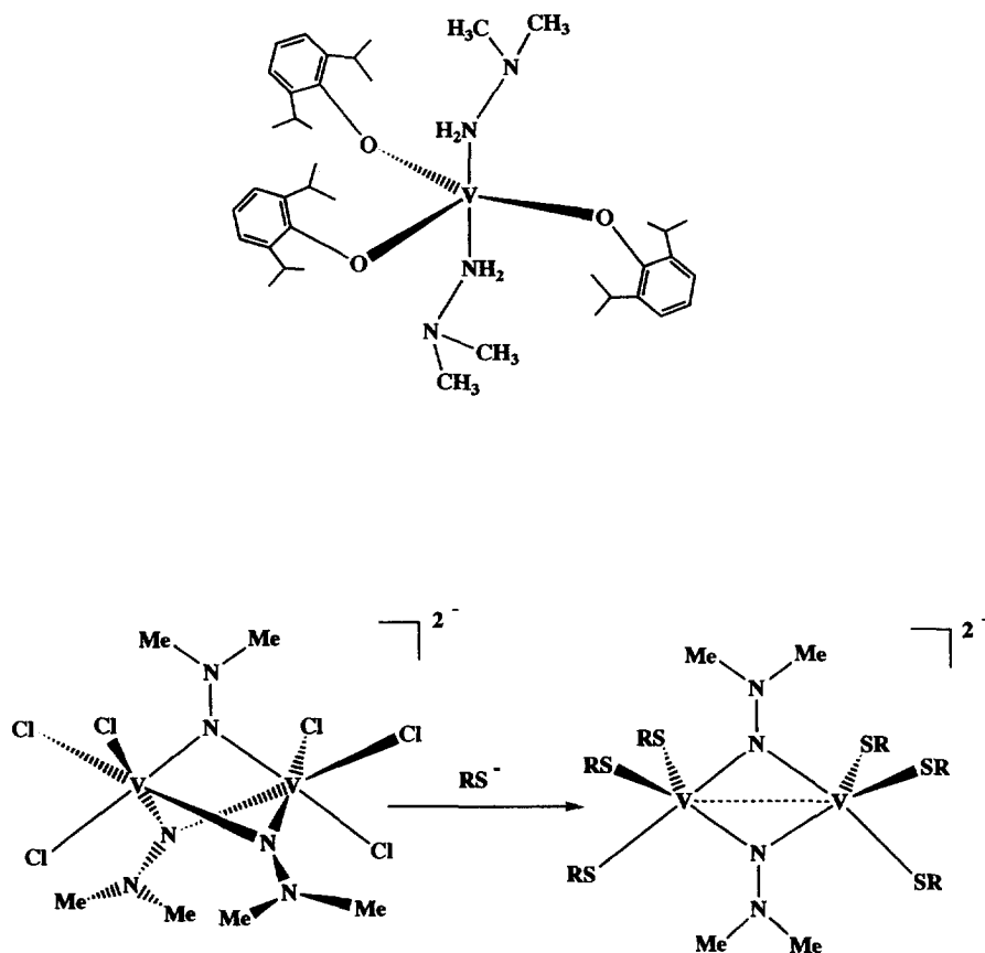
Fig. 11. Hydrazine and hydrazide complexes of vanadium.
