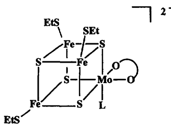
Fig. 8. Cluster anions which model the coordination environment of Mo in FeMoco ( \text{L} = \text{MeCN} , imidazole, etc.; \text{O}=\text{O} = \text{C}_6\text{Cl}_4\text{O}_2^{2-} )
