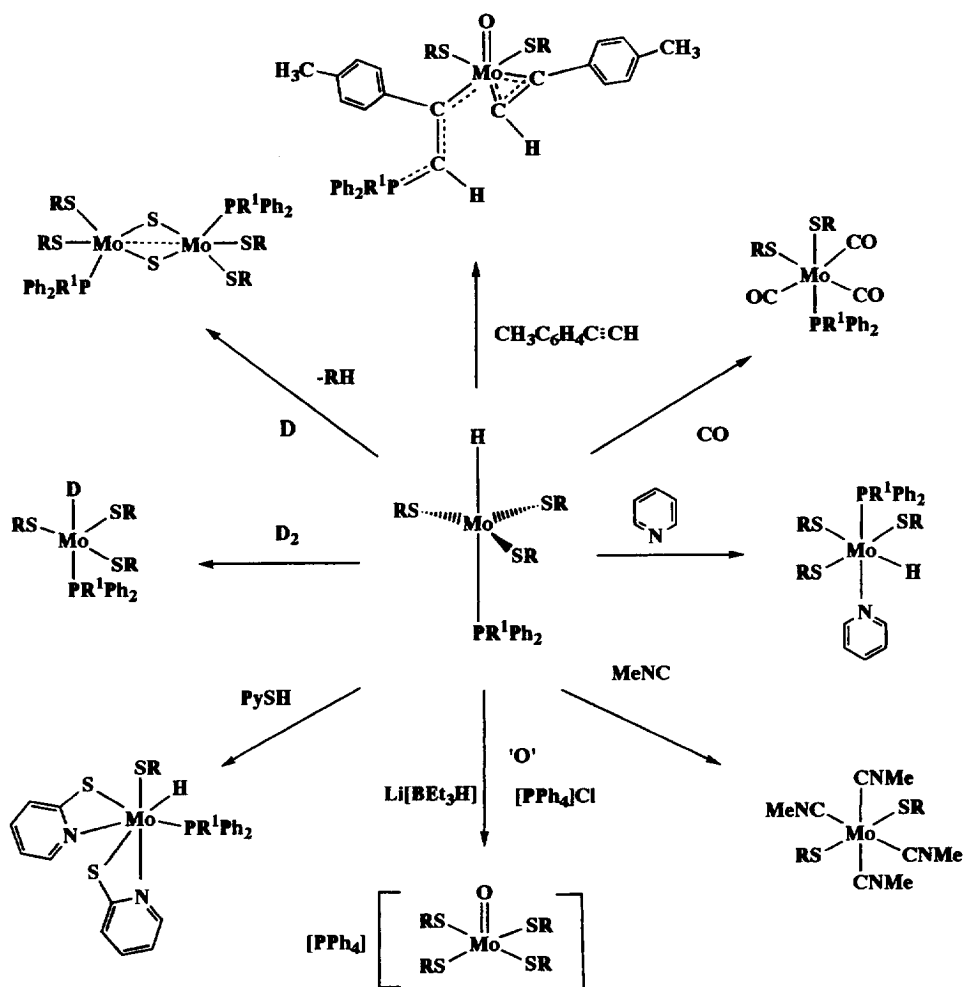
Fig. 9. General scheme of reactions of the complexes [\text{MoH}(\text{SR})_3(\text{PR}^1\text{Ph}_2)] ( \text{R} = \text{C}_6\text{H}_2\text{Me}_3\text{-2,4,6} or \text{C}_6\text{H}_2\text{Pr}_3\text{-2,4,6} ; \text{R}^1 = \text{Me} or \text{Et} ).
