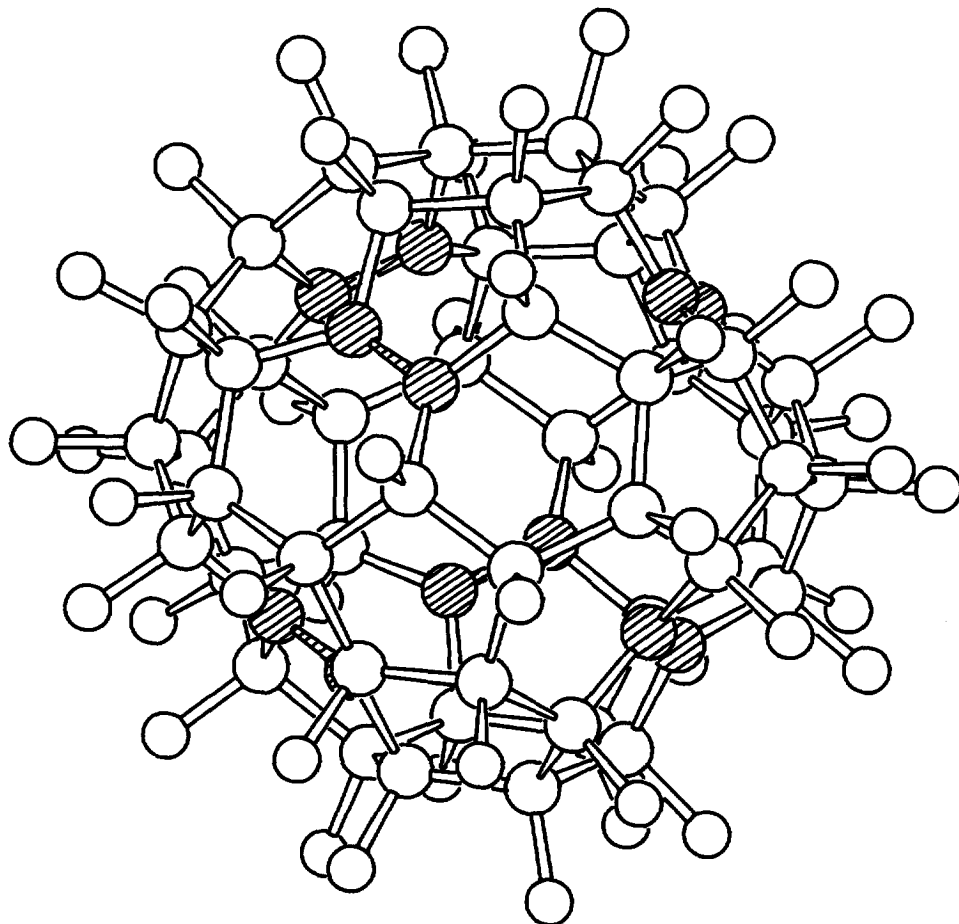
Fig. 23. The D_3 isomer of C_{60}F_{48} . The three-fold axis is from the top to the bottom of the figure. For clarity, the C=C carbon atoms and bonds are hatched.
