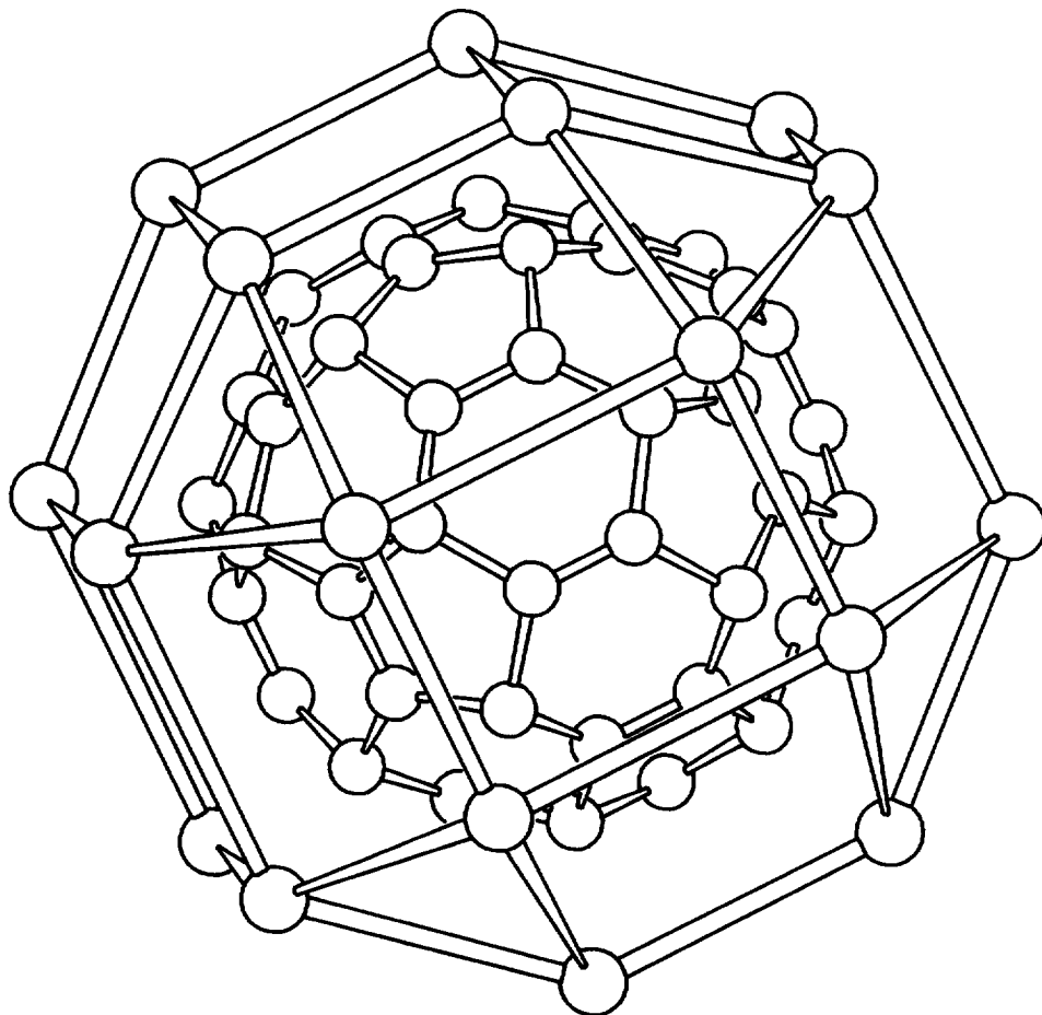
Fig. 20. The structure of C_{60}Br_{24} showing a rhombicuboctahedral arrangement of 24 bromine atoms outside a truncated icosahedral arrangement of 60 carbon atoms.
