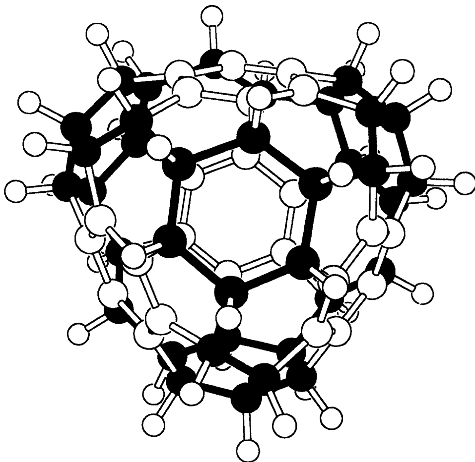
Fig. 8. Structure of C_{60}H_{36} (first series) viewed down the three-fold axis. For clarity, the HC–CH carbon atoms and bonds are shaded.
