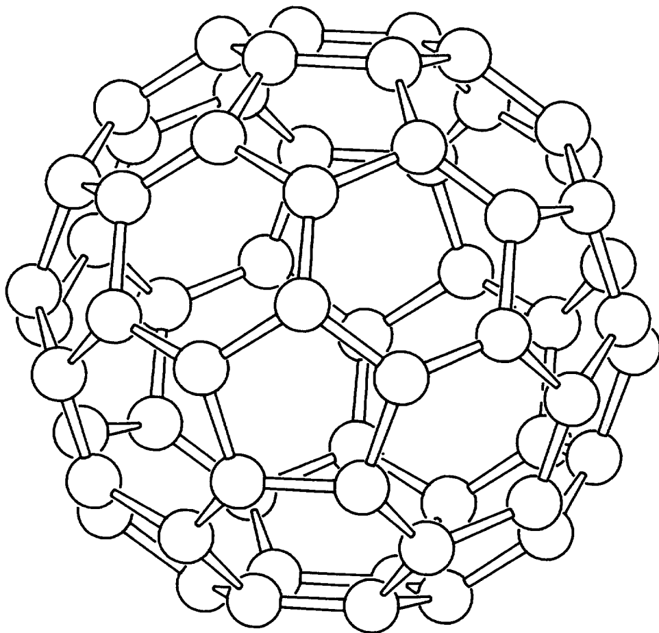
Fig. 1. The truncated icosahedral structure of C_{60} .
