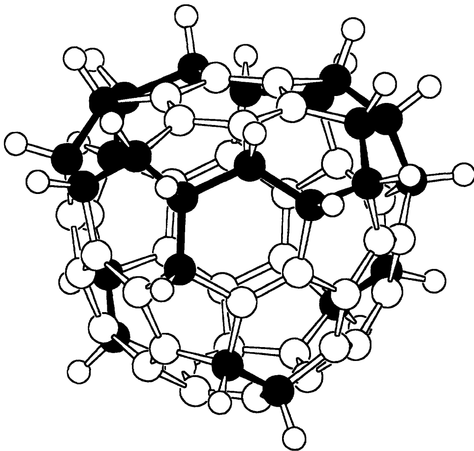
Fig. 6. Structure of C_{60}H_{24} (first series). For clarity, the HC–CH carbon atoms and bonds are shaded. The molecule is drawn in the same orientation as for C_{60}H_{12} (Fig. 4) and C_{60}H_{16} (Fig. 5).
