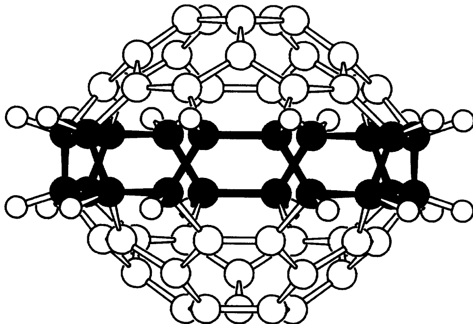
Fig. 12. D_{5d} structure of C_{60}H_{20} . For clarity, the HC-CH carbon atoms and bonds are shaded.
