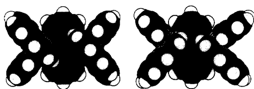
\Lambda,\Lambda - and \Lambda,\Delta -isomers of the compound [(\text{Ru}(\text{phen})_2)(\text{bipym})]^{4+}
