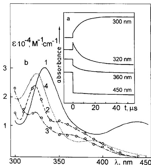
Fig. 4. (a) Kinetic changes in the optical density of \text{Ni(dtc)}_3^+ solution ( 3 \times 10^{-4} \text{ M} ) in acetonitrile at 295 K after the laser pulse (532 nm; cuvette 1 mm). (b) Spectra of the intermediates arising in succession: (1) spectrum before the pulse (initial spectrum); (2,3) spectra 1 \mu\text{s} and 50 \mu\text{s} after the pulse, respectively; (4) final spectrum. Adapted from Ref. [55].
