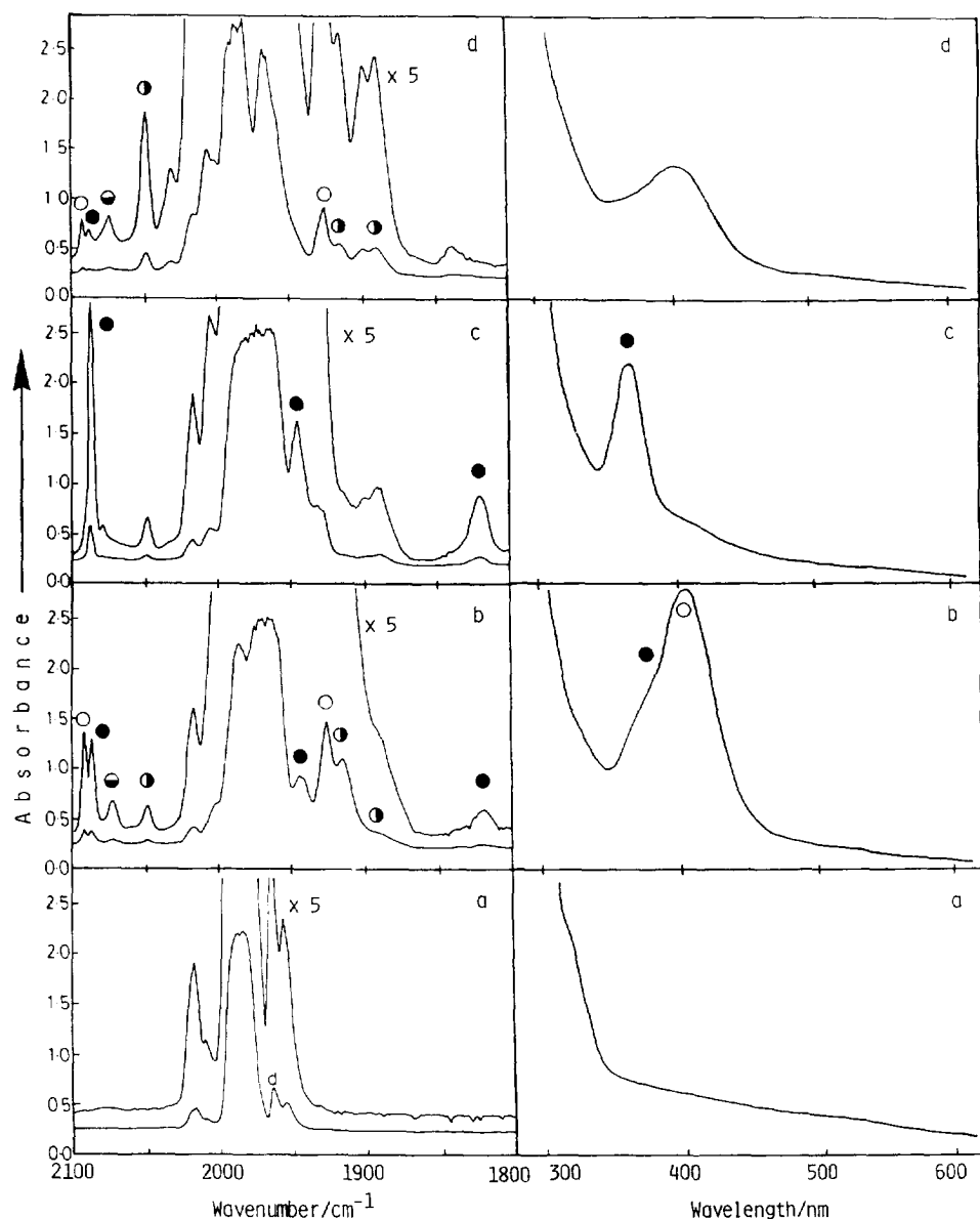
Fig. 1. IR absorption spectrum in the region 1800–2100 cm -1 and UV-vis absorption spectrum in the region 300–600 nm displayed by a solid CH 4 matrix containing Mo(CO) 6 and C 2 H 2 with the composition Mo(CO) 6 :C 2 H 2 :CH 4 of ca. 1:100:2000 at 20 K showing the effects of short-term photolysis at different wavelengths. (a) Spectra of the matrix after deposition. (b) Spectra after photolysis at λ=313 nm. (c) Spectra after photolysis at λ=445 nm. (d) Spectra after photolysis at λ=369 nm. Bands are labelled as follows: ○ [CH 4 ⋯Mo(CO) 5 ]; ● [(η 2 -C 2 H 2 )Mo(CO) 5 ]; ◐ [H 2 C=C=Mo(CO) 5 ]; ◑ Mo(CO) 4 ; 'd' [HC≡CH] 2 . (Reproduced with permission from Ref. [25]).
