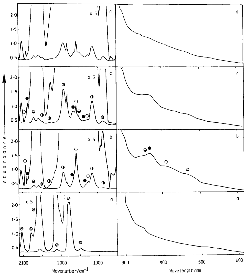
Fig. 2. IR absorption spectrum in the region 1850\text{--}2100\text{ cm}^{-1} and UV-vis absorption spectrum in the region 300\text{--}600\text{ nm} displayed by a solid \text{CH}_4 matrix containing \text{W}(\text{CO})_6 and \text{MeC}\equiv\text{CH} with the composition \text{W}(\text{CO})_6:\text{MeC}\equiv\text{CH}:\text{CH}_4 of ca. 1:250:5000 at 20\text{ K} showing the effects of short-term photolysis at different wavelengths. (a) Spectra of the matrix after deposition. (b) Spectra after photolysis at \lambda=445\text{ nm} . (c) Spectra after photolysis at \lambda=369\text{ nm} . (d) Spectra after photolysis at \lambda=313\text{ nm} . Bands are labelled as follows: \circ [\text{CH}_4\cdots\text{W}(\text{CO})_5] ; \bullet [(\eta^2\text{-MeC}\equiv\text{CH})\text{W}(\text{CO})_3] ; \circ [\text{Me}(\text{H})\text{C}=\text{C}=\text{W}(\text{CO})_3] ; \blacksquare \text{W}(\text{CO})_4 species; \square free [\text{MeCCH}] or [\text{MeCCH}]_n ; and \otimes [\text{W}(\text{CO})_6] . (Reproduced with permission from Ref. [26]).
