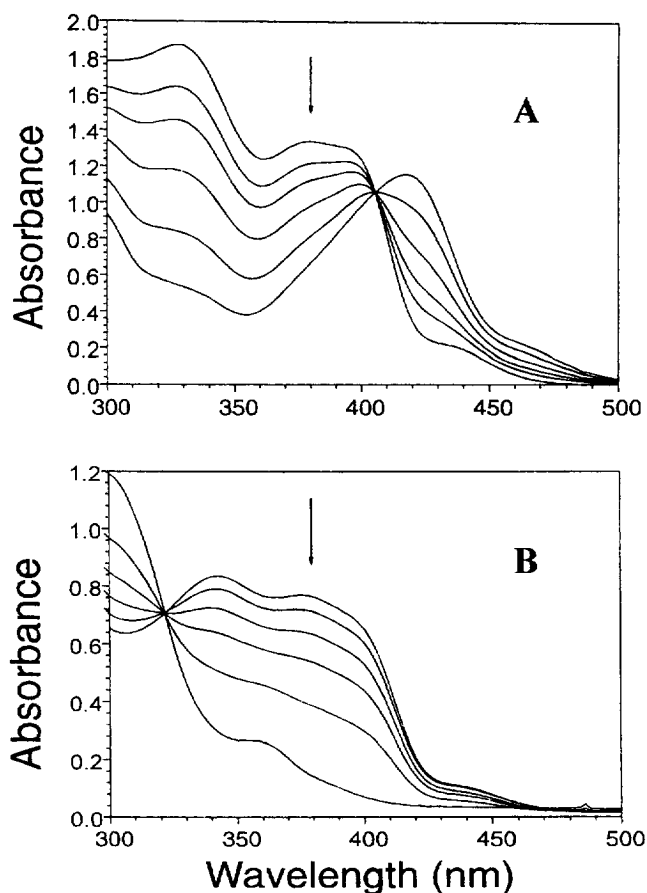
Fig. 1. Spectral changes during photolysis of \text{W(CO)}_5\text{py} in (A) methanol and (B) 24:1 chloroform–1-hexene.
