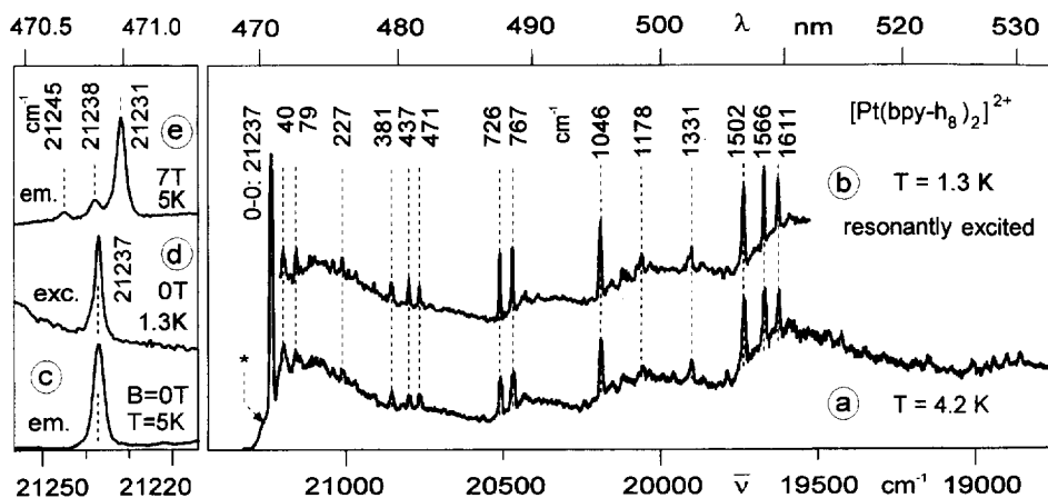
Fig. 5. Highly resolved emission of a [\text{Pt}(\text{bpy}-\text{h}_8)_2]^{2+} trap in neat [\text{Pt}(\text{bpy}-\text{h}_8)_2](\text{ClO}_4)_2 (see Ref. [75]). (a) Excitation energy \bar{\nu}_{\text{exc}} = 21\,839 \text{ cm}^{-1} ( \approx 457.9 \text{ nm} ). The asterisk characterizes an emission from higher-lying trap(s). (b) Resonantly excited emission ( \bar{\nu}_{\text{exc}} = 21\,237 \text{ cm}^{-1} , electronic origin S_0 \rightarrow T_1 ). (c)–(e) Region of the electronic origin(s) on an enlarged scale. The excitation (d) is detected at 19\,626 \text{ cm}^{-1} ( \approx 1611 \text{ cm}^{-1} satellite). The crystals were grown from DMF.
