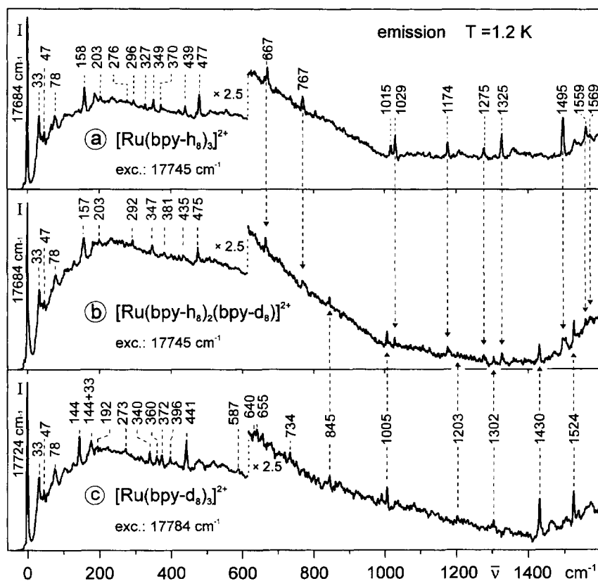
Fig. 10. Emission spectra of [\text{Ru}(\text{bpy-h}_8)_3]^{2+} , [\text{Ru}(\text{bpy-h}_8)_2(\text{bpy-d}_8)]^{2+} , and [\text{Ru}(\text{bpy-d}_8)_3]^{2+} in [\text{Zn}(\text{bpy-h}_8)_3](\text{ClO}_4)_2 at T = 1.2 K (see Ref. [21]). The spectra are selectively excited into the respective electronic origins I. The wavenumber scale gives the separation from the lowest electronic origin I. For further data see Fig. 9. Note that [\text{Ru}(\text{bpy-h}_8)_2(\text{bpy-d}_8)]^{2+} exhibits vibrational satellites, which correspond to both types of ligand. This is very strong evidence for delocalization in the lowest excited state.
