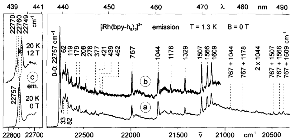
Fig. 2. Highly resolved and line-narrowed emission of [\text{Rh}(\text{bpy-h}_8)_3]^{3+} in [\text{Zn}(\text{bpy-h}_8)_3](\text{ClO}_4)_2 (see Ref. [42]). The excitation energy for (a) and (c) was \bar{\nu}_{\text{exc}} = 29\,665 \text{ cm}^{-1} ( \approx 337.1 \text{ nm} ), and for the line-narrowed spectrum (b) was \bar{\nu}_{\text{exc}} = 22\,757 \text{ cm}^{-1} ( S_0 \rightarrow T_1 , resonantly excited). The crystals were grown from water/acetone (1:4) with a solution molar ratio Rh(III):Zn(II) of 1%. The energies of the satellites are specified relative to the electronic origin at 22\,757 \text{ cm}^{-1} . (c) shows the region of the origin(s) on an enlarged scale for B = 0 \text{ T} and B = 12 \text{ T} , respectively ( T = 20 \text{ K} ).
