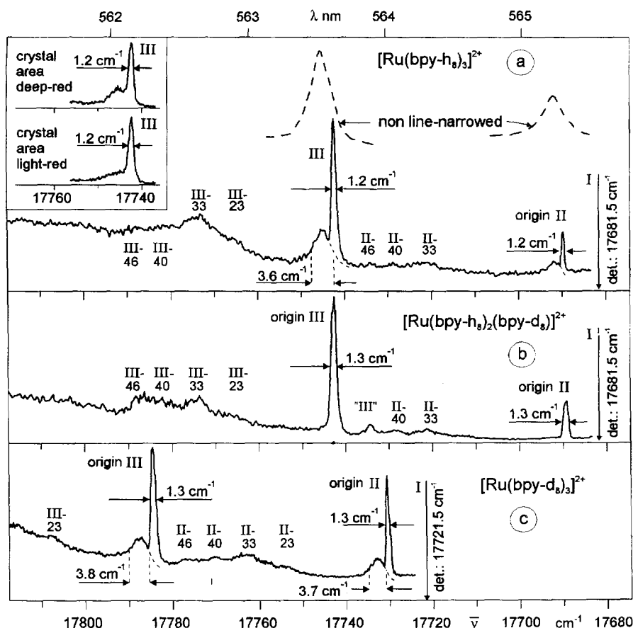
Fig. 11. Line-narrowed excitation spectra at T=1.2 \text{ K} of [\text{Ru}(\text{bpy-h}_8)_3]^{2+} , [\text{Ru}(\text{bpy-h}_8)_2(\text{bpy-d}_8)]^{2+} , and [\text{Ru}(\text{bpy-d}_8)_3]^{2+} in [\text{Zn}(\text{bpy-h}_8)_3](\text{ClO}_4)_2 . The crystals were grown from aqueous solutions having molar ratios \text{Ru(II)}:\text{Zn(II)} of 0.5% (a, b); 0.3% (c); 0.03% (inset). The spectra show the electronic origins II and III and the corresponding phonon satellites. Detection is at the energy of the respective electronic origin I. Peak "III'" represents an unavoidable artefact; see text. Inset: the excitation structures of the electronic origin III (same \text{cm}^{-1} scale) measured at two positions of the same crystal. The spectral change displays the differences in clustering of the [\text{Ru}(\text{bpy})_3]^{2+} chromophores (see Section 4.1). It is important to note that [\text{Ru}(\text{bpy-h}_8)_2(\text{bpy-d}_8)]^{2+} exhibits the same number of electronic origins as found for the per-compounds.
