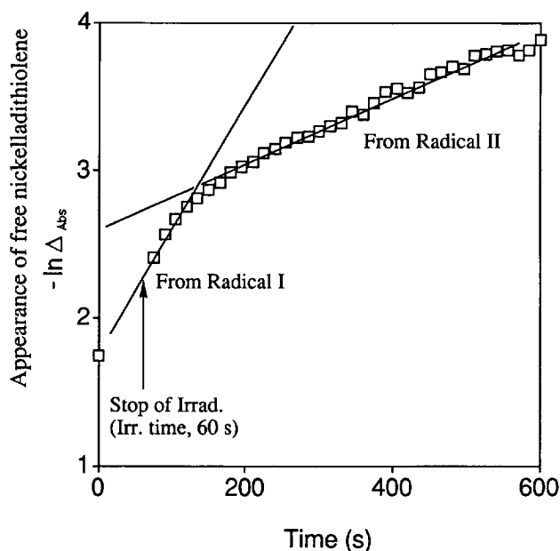
Fig. 2. Logarithmic plot of appearance of free nickeladithiolene from the intermediates in the photolysis of S,S' -butane-1,4-diyl derivatives of bis(1,2-diphenyl-1,2-ethenedithiolato)nickel.
