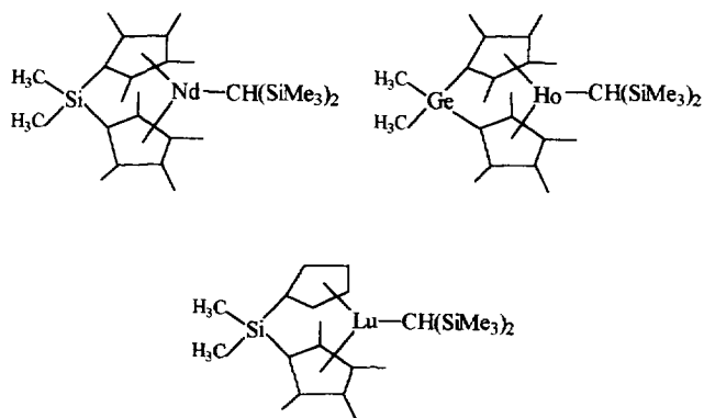
Fig. 25. The structure of ring bridged [\{\text{Me}_2\text{Si}(\text{C}_5\text{Me}_4)_2\}\text{Nd}(\text{CH}(\text{SiMe}_3)_2)] , [\{\text{Me}_2\text{Ge}(\text{C}_5\text{Me}_4)_2\}\text{Ho}(\text{CH}(\text{SiMe}_3)_2)] and [\{\text{R}_2\text{Si}(\text{C}_5\text{Me}_4)(\text{C}_5\text{H}_4)\}\text{Lu}(\text{CH}(\text{SiMe}_3)_2)] .
