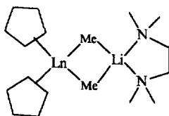
Fig. 20. The structure of [Cp 2 Ln( \mu -Me) 2 Li(tmed)].
