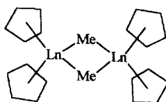
Fig. 19. The structure of [\text{Cp}_2\text{Ln}(\mu\text{-Me}_2)\text{LnCp}_2] .
