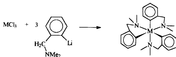
Fig. 12. The structure of [M(o-C_6H_4CH_2NMe_2)_3] ( M = Er, Yb, Lu ).
