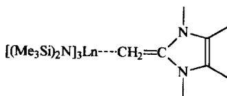
Fig. 30. The structure of the carbene complex [\text{Ln}(\text{N}(\text{SiMe}_3)_2)_3(1,3,4,5\text{-tetramethyl-2-methyleneimidazoline})] .
