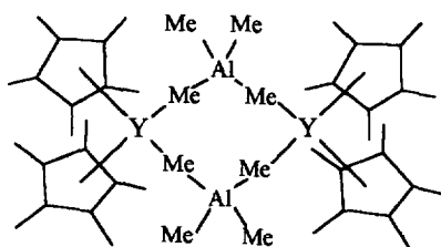
Fig. 24. The structure of [\text{Cp}^*_2\text{Y}(\mu\text{-Me}_2\text{AlMe}_2)_2\text{YCp}^*] .
