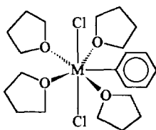
Fig. 2. The structure of \text{PhGdCl}_2 \cdot 4\text{THF} .
