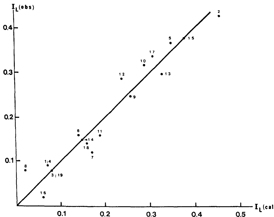
Fig. 14. Plot of observed versus calculated ligand intensity I_L (see Table 1 for numbering) (from Ref. [71]).
