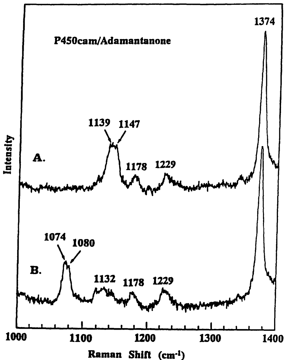
Fig. 20. Resonance Raman spectra of dioxygen adduct of adamantanone-bound cytochrome P450 cam at -80^{\circ}\text{C} in the \nu(\text{O}-\text{O}) region: trace A, ^{16}\text{O}_2 ; trace B, ^{18}\text{O}_2 . Excitation at 413.1 nm (from Ref. [96]).
