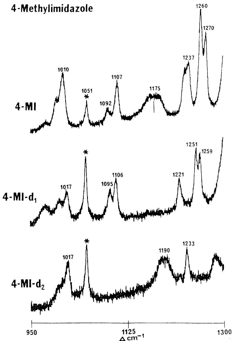
Fig. 5. Raman spectra of 4-methylimidazole and deuteriated analogues (see text) in C 2 H 2 Cl 2 measured at room temperature with excitation at 406.7 nm (10 mW of laser power at the sample). Asterisks mark solvent bands (from Ref. [67]).
