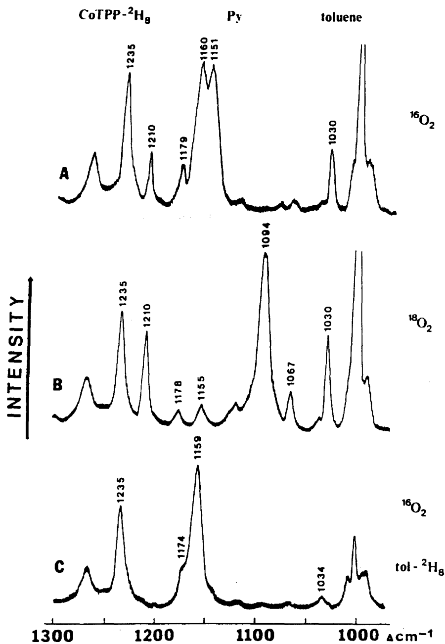
Fig. 15. Resonance Raman spectra of \text{Co}(\text{TPP-}^2\text{H}_8) in toluene containing 3% pyridine at -85^\circ\text{C} under \sim 4 atm of \text{O}_2 pressure: (A) ^{16}\text{O}_2 ; (B) ^{18}\text{O}_2 ; (C) ^{16}\text{O}_2 , toluene- ^2\text{H}_8 (from Ref. [84]).
