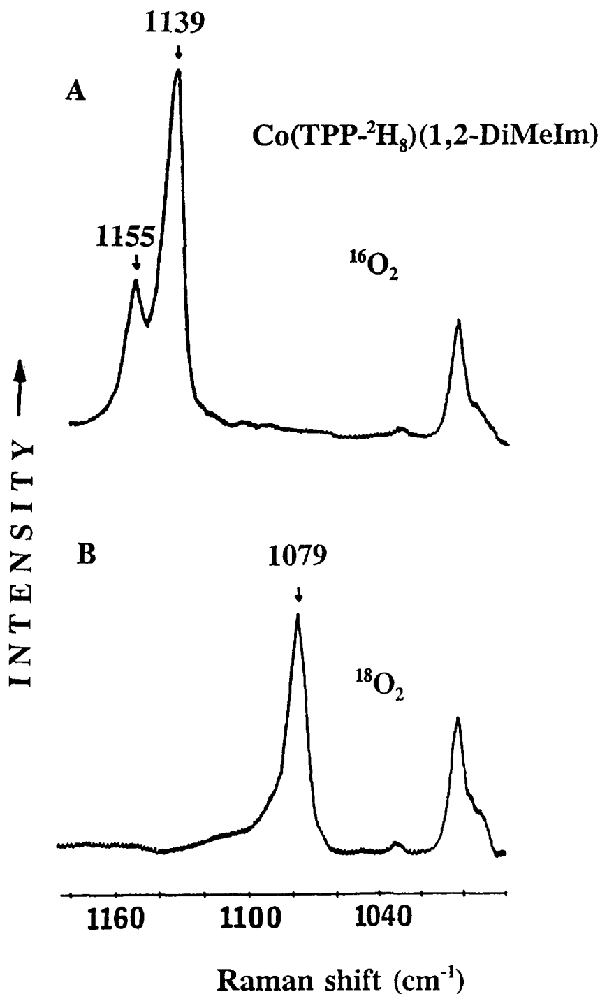
Fig. 3. Resonance Raman spectra (406.7-nm excitation) of dioxygen adducts of \text{Co(TPP-}^2\text{H}_8\text{)} in \text{CH}_2\text{Cl}_2 containing 3% of 1,2-dimethylimidazole at -90^\circ\text{C} under ca. 4 atm. of \text{O}_2 pressure: (A) ^{16}\text{O}_2 ; (B) ^{18}\text{O}_2 (adapted from Ref. [60]).
