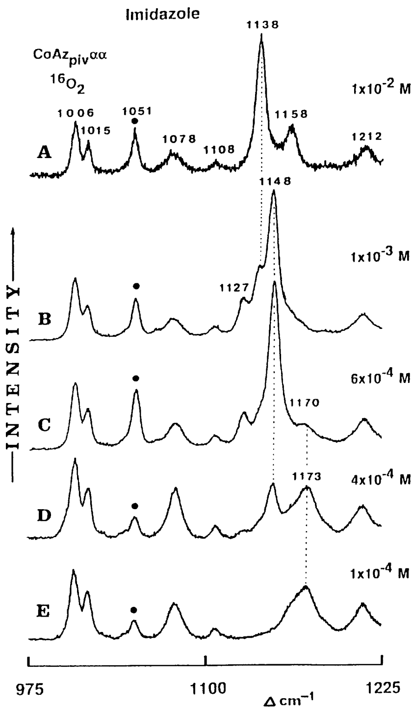
Fig. 10. Influence of imidazole concentration on resonance Raman spectra of the 16 O 2 adduct of CoAz piv αα complex with imidazole. Temperature at ~185 K. Spectral conditions as in Fig. 8 (from Ref. [77]).
