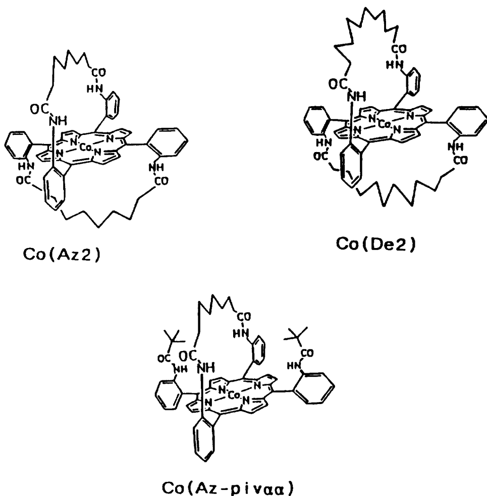
Fig. 12. Structures of Co(Az2), Co(De2) and Co(Az pivaa ).
