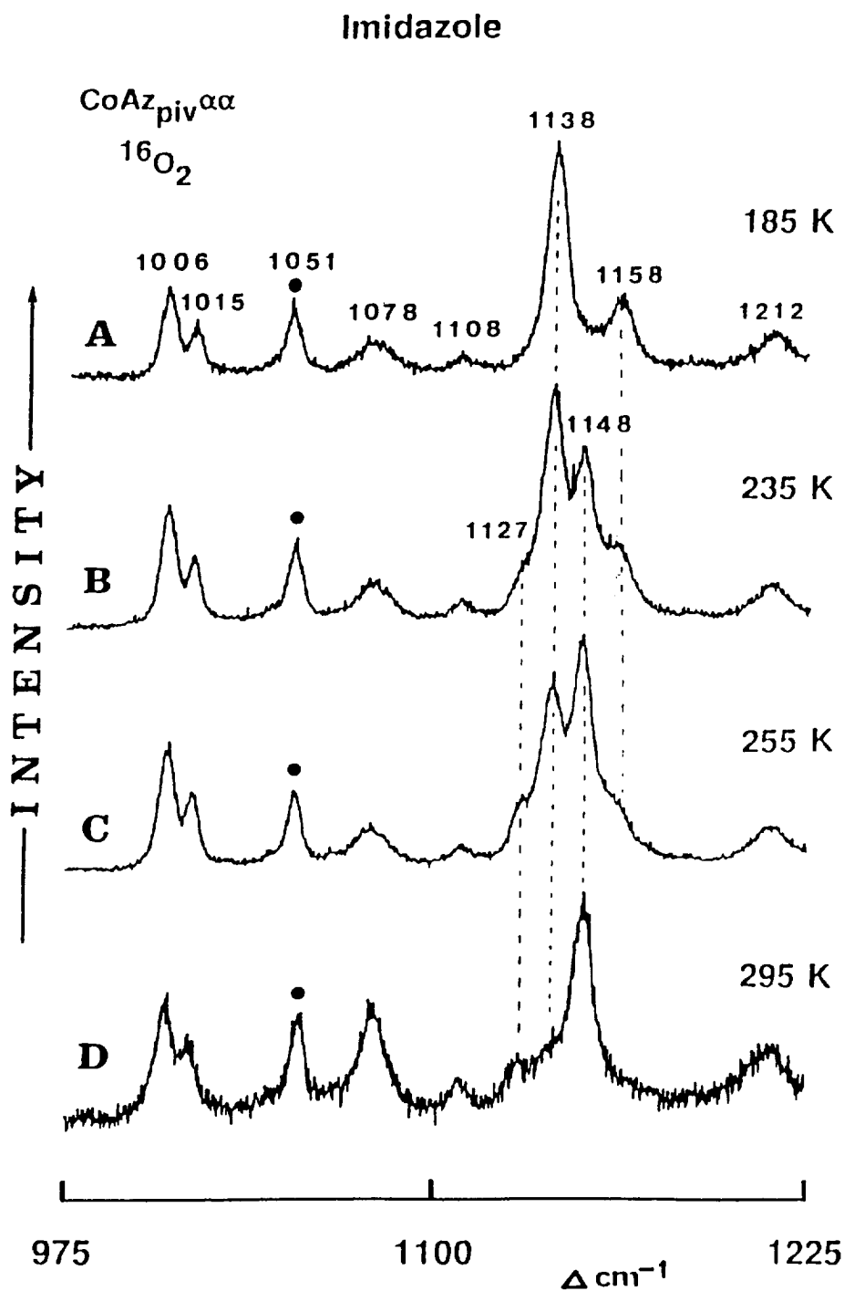
Fig. 9. Influence of temperature on resonance Raman spectra of the ^{16}\text{O}_2 adduct of \text{CoAz}_{\text{piv}}\alpha\alpha complex with imidazole. Spectral conditions as in Fig. 8 (from Ref. [77]).
