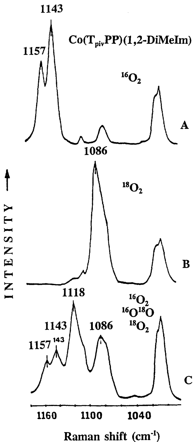
Fig. 4. Resonance Raman spectra (406.7-nm excitation) of dioxygen adducts of \text{Co}(\text{T}_{\text{pivPP}}) in \text{CH}_2\text{Cl}_2 containing 3% of 1,2-dimethylimidazole at -90^\circ\text{C} under ca. 4 atm. of \text{O}_2 pressure: (A) ^{16}\text{O}_2 ; (B) ^{18}\text{O}_2 ; (C) ^{16}\text{O}_2/^{16}\text{O}^{18}\text{O}/^{18}\text{O}_2 = 1/2/1 (adapted from Ref. [60]).
