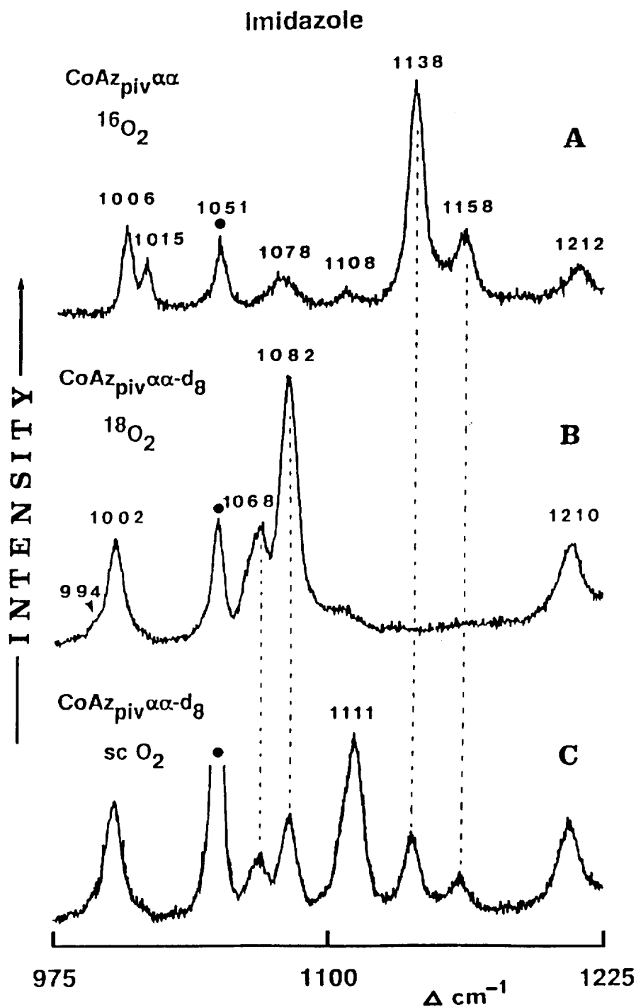
Fig. 8. Resonance Raman spectra of O 2 adducts of CoAz piv αα complex with imidazole. Excitation at 406.7 nm (~10 mW of laser power at the sample). The 1051 cm -1 band is due to C 2 H 2 Cl 2 (from Ref. [77]).
