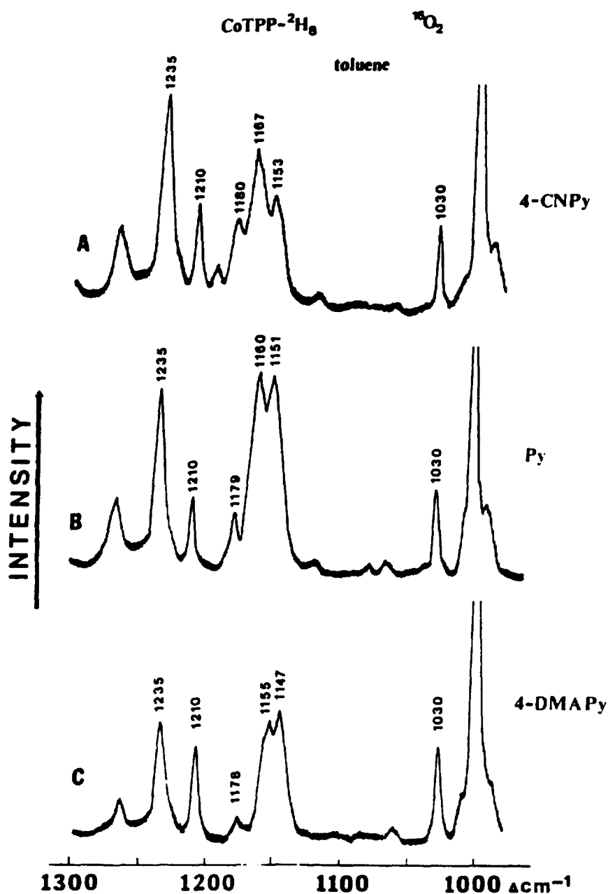
Fig. 16. Resonance Raman spectra of \text{Co(TPP-}^2\text{H}_8\text{)} in toluene containing 3% 4-cyanopyridine (A), pyridine (B), and 4-dimethylaminopyridine (C) at -85^\circ\text{C} under \sim 4 atm of ^{16}\text{O}_2 pressure (from Ref. [84]).
