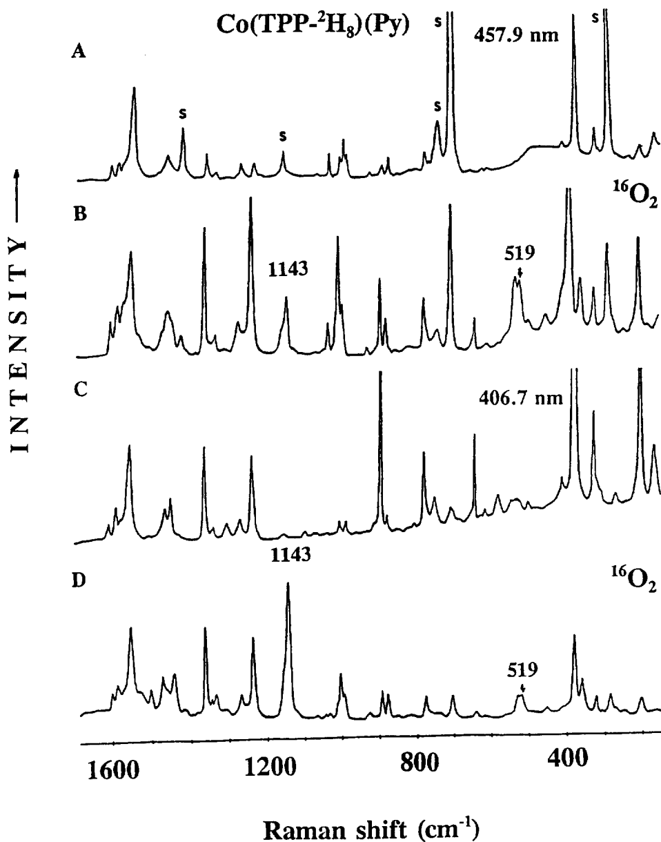
Fig. 1. Resonance Raman spectra of Co(TPP- 2 H 8 ) in CH 2 Cl 2 solution containing 3% pyridine at -90°C: (A) Co(TPP- 2 H 8 ) + no oxygen, 457.9-nm excitation; (B) Co(TPP- 2 H 8 ) + 16 O 2 (ca. 4 atm.), 457.9-nm excitation; (C) Co(TPP- 2 H 8 ) + no oxygen, 406.7-nm excitation; (D) Co(TPP- 2 H 8 ) + 16 O 2 (ca. 4 atm.), 406.7-nm excitation. "S" denotes the solvent bands (adapted from Ref. [60]).
