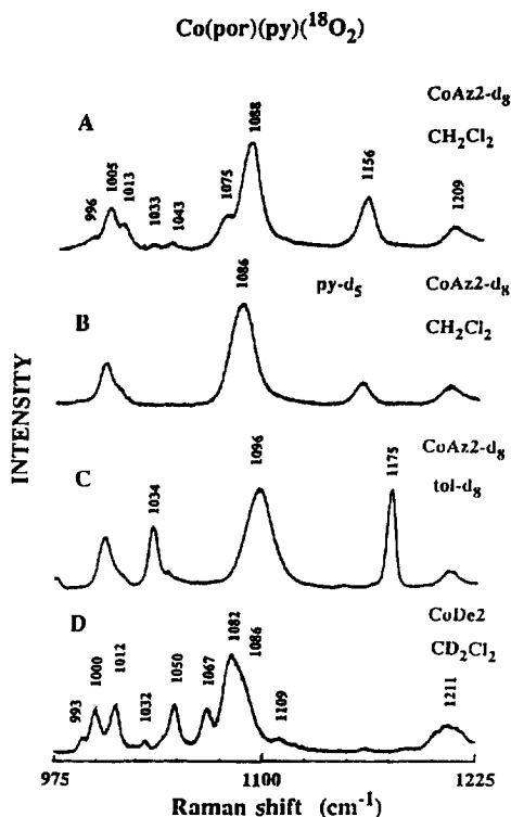
Fig. 13. Resonance Raman spectra of 18 O 2 adducts of Co(porphyrin)(py) complexes (excitation at 406.7 nm): (A) CoAz2-d 8 , CH 2 Cl 2 ; (B) CoAz2-d 8 , CH 2 Cl 2 ; (C) CoAz2-d 8 , tol-d 8 ; (D) CoDe2, CD 2 Cl 2 (from Ref. [61]).
