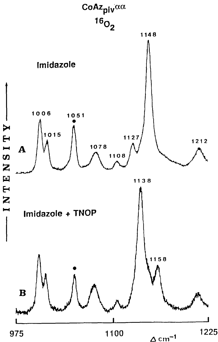
Fig. 11. Resonance Raman spectra of the ^{16}\text{O}_2 adduct of \text{CoAz}_{\text{piv}}^{\alpha\alpha} complex with imidazole. The effect of tri- n -octylphosphine oxide (TNOP); imidazole concentration \sim 1 \times 10^{-3} M, TNOP concentration \sim 5 \times 10^{-2} M. Temperature in both experiments \sim 185 K. Spectral conditions as in Fig. 8 (from Ref. [77]).
