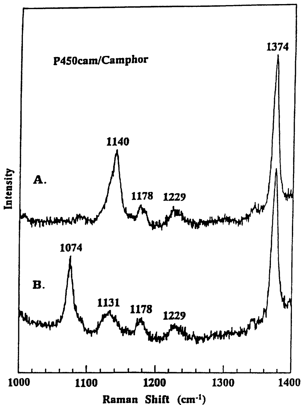
Fig. 19. Resonance Raman spectra of dioxygen adduct of camphor-bound cytochrome P450 cam in the \nu(\text{O}-\text{O}) region: trace A, ^{16}\text{O}_2 ; trace B, ^{18}\text{O}_2 . Excitation at 413.1 nm (from Ref. [96]).
