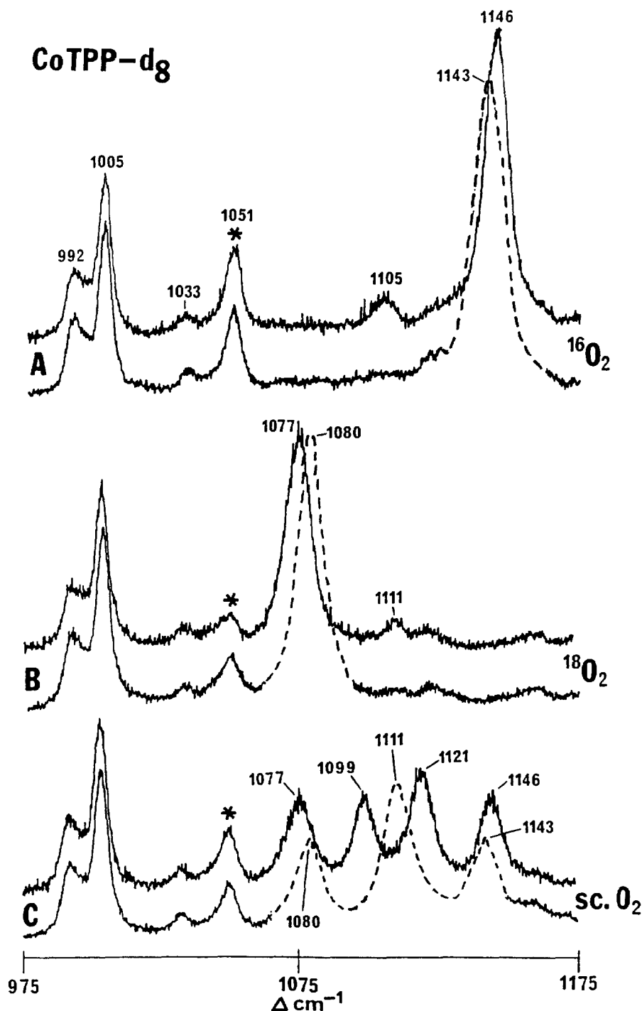
Fig. 6. Resonance Raman spectra of dioxygen adducts of Co(TPP- 2 H 8 ) in the presence of 4-MI (solid line) or 4-MI- 2 H 2 (dashed line) at -90°C in C 2 H 2 Cl 2 with excitation at 406.7 nm (10 mW of laser power at the sample): (A) 16 O 2 ; (B) 18 O 2 ; (C) 16 O 2 16 O 18 O/ 18 O 2 (1/2/1). Asterisks mark solvent bands (from Ref. [67]).
