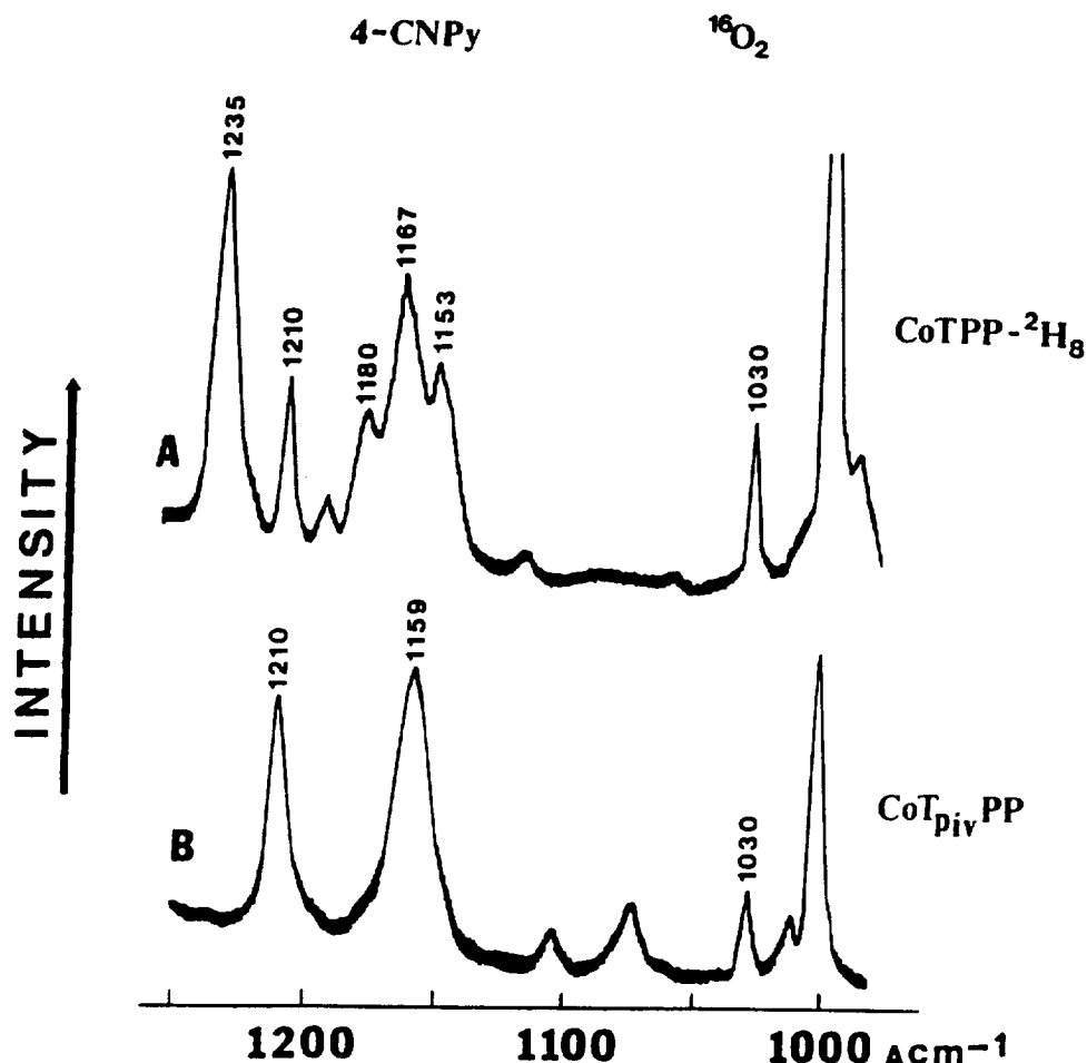
Fig. 17. Resonance Raman spectra of Co(TPP-²H₈) (trace A) and \alpha^4 -Co(T piv PP) (trace B) in toluene containing 3% 4-cyanopyridine at -85°C under ~4 atm of ¹⁶O₂ pressure (from Ref. [84]).
