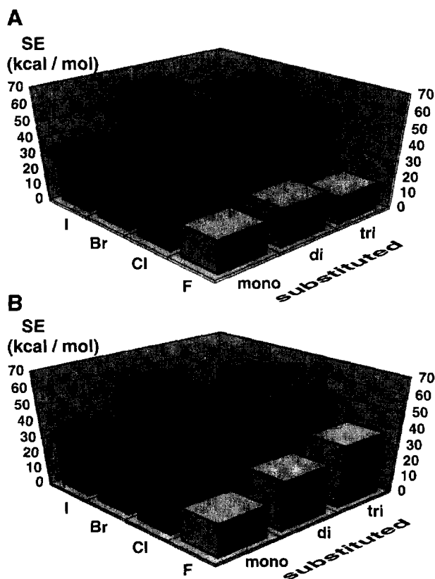
Fig. 7. Graphical representation of experimentally determined values of the stabilization energies SE (in \text{kcal mol}^{-1} ) for the cations X_n\text{CH}_3^{\oplus-n} ( X=\text{F}, \text{Cl}, \text{Br}, \text{I} ). Data shown in (A) are calculated according to the isodesmic reaction: X_n\text{CH}_3^{\oplus-n} + \text{CH}_4 \rightarrow X_n\text{CH}_{4-n} + \text{CH}_3^{\oplus} according to \Delta H_f(X_n\text{CH}_{4-n}) + \Delta H_f(\text{CH}_3^{\oplus}) - \Delta H_f(\text{CH}_4) - \Delta H_f(X_n\text{CH}_3^{\oplus-n}) . Data shown in (B) are calculated according to the isodesmic reaction: X_n\text{CH}_3^{\oplus-n} + n\text{CH}_4 \rightarrow nX\text{CH}_3 + \text{CH}_3^{\oplus} according to (n \cdot \Delta H_f(X_n\text{CH}_{4-n})) + \Delta H_f(\text{CH}_3^{\oplus}) - (n \cdot \Delta H_f(\text{CH}_4)) - \Delta H_f(X_n\text{CH}_3^{\oplus-n}) .
