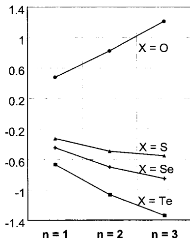
Fig. 3. Graphical representation of total charges on the carbon center of (HX)_nCH_3^{\oplus-n} based on NPA calculations at MP2(full)/LANLIDZ+P' level.
