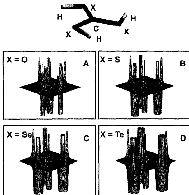
Fig. 5. Three-dimensional plot of Laplacians -\nabla^2\rho(r) (in a.u.) for (HX)_3C^\oplus for the plane including all nuclei. The orientation of the cations is shown on top. (A) (HO)_3C^\oplus ; (B) (HS)_3C^\oplus ; (C) (HSe)_3C^\oplus ; (D) (HTe)_3C^\oplus .
