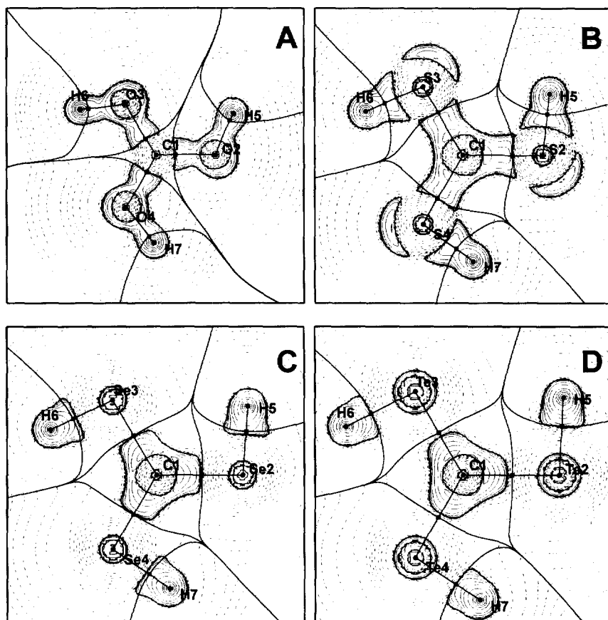
Fig. 6. Two-dimensional plot of Laplacians -\nabla^2\rho(r) (in a.u.) for (HX)_3C^\oplus for the plane including all nuclei. Solid lines indicate charge concentration, dashed lines charge depletion. Interatomic zero-flux surfaces and bond paths are shown as solid bold lines. Bond critical points are indicated by squares (■). (A) (HO)_3C^\oplus ; (B) (HS)_3C^\oplus ; (C) (HSe)_3C^\oplus ; (D) (HTe)_3C^\oplus .
