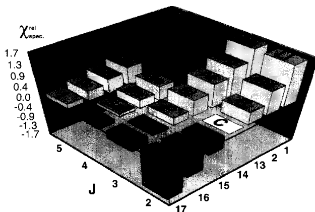
Fig. 1. Relative spectroscopic electronegativities, \chi_{\text{spec}}^{\text{rel}} , of group 1–2 and 13–17 elements which were considered as \alpha -heteroatoms in carbenium ions (\text{RX})_n\text{CH}_3^{\oplus-n} .
