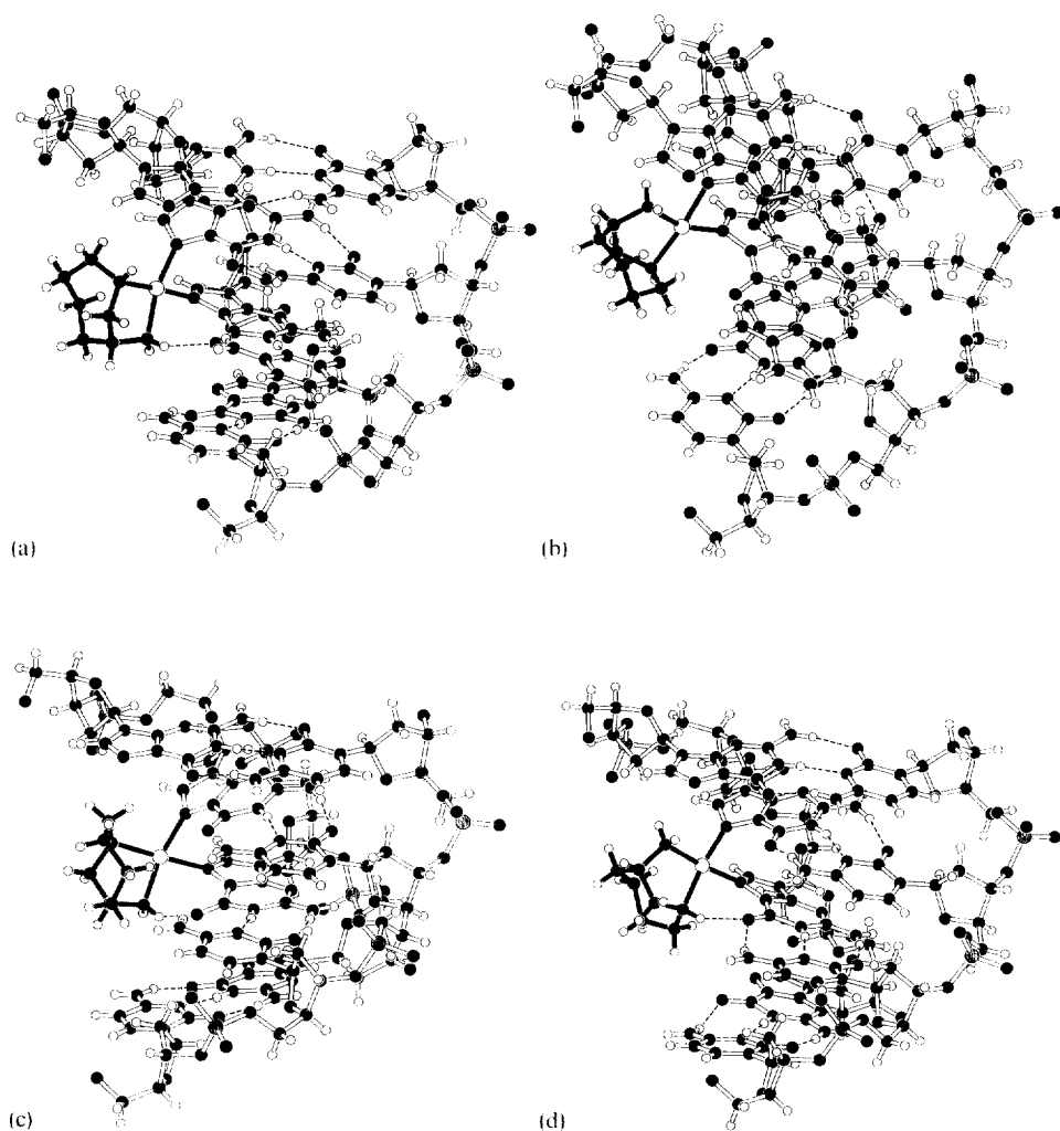
Fig. 13. Views of the molecular mechanics models of the isomers of the intrastrand adducts formed between \text{Pt(ahaz)}_2^{2+} and (5'-d(GpGpGpG*pG*pGpGpG)-3', 5'-d(CpCpCpCpCpCpC)-3').
