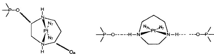
Fig. 7. Schematic diagrams of intrastrand and interstrand adducts demonstrating the logic behind the design of [\text{Pt}(\text{hpic})\text{Cl}_2] .
