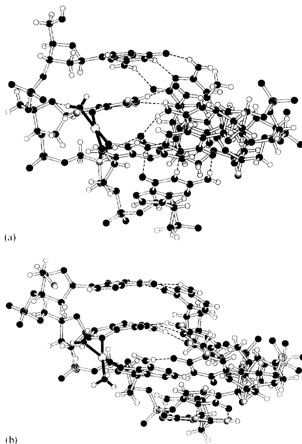
Fig. 2. (a) Molecular mechanics model of \text{Pt}(\text{NH}_3)_2 : (5'-d(GpA*pG*pG)-3', 5'-d(CpCpTpC)-3'). (b) Molecular mechanics model of \text{Pt}(\text{NH}_3)_2 : (5'-d(GpG*pA*pG)-3', 5'-d(CpTpCpC)-3').
