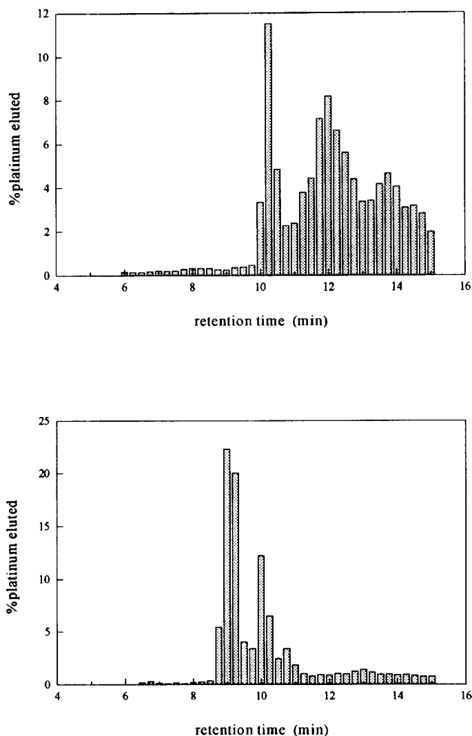
Fig. 4. Adduct profile for the binding of 39 (a) and [Pt(en)Cl 2 ] (b) to salmon-sperm DNA.
