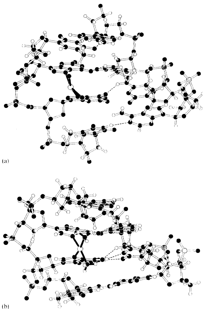
Fig. 1. (a) Central four base pairs from the crystal structure of \text{Pt}(\text{NH}_3)_2 : (5'-d(CpCp(Br)UpCpTpG*pG*pTpCpTpCpC)-3', 5'-d(GpGpApGpApCpCpApGpApGpG)-3') [82]. (b) Central four base pairs from the molecular mechanics model of \text{Pt}(\text{NH}_3)_2 : (5'-d(TpCpTpG*pG*pTpCpTp)-3', 5'-d(ApGpApCpCpApGpAp)-3').
