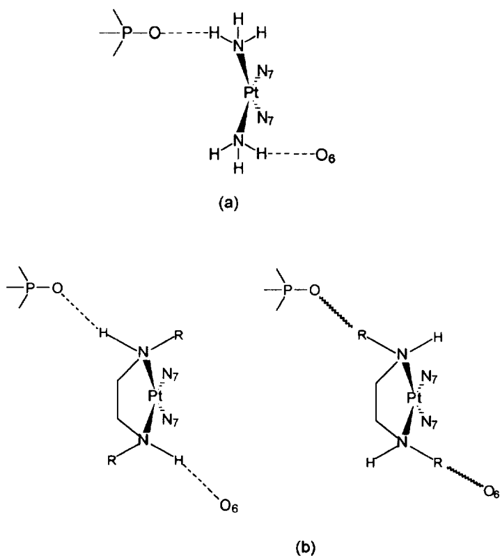
Fig. 9. Schematic diagrams of intrastrand and interstrand adducts demonstrating the logic behind the design of chiral Pt complexes.
