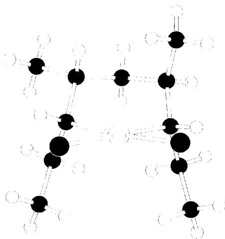
Fig. 10. Crystal structure of [\text{Pt}(\text{R},\text{R-eap})\text{Cl}_2] .
