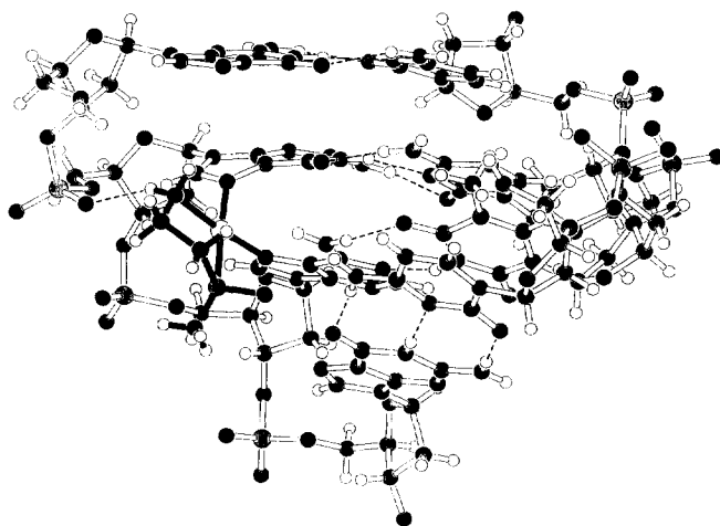
Fig. 3. Molecular mechanics model of \text{Pt}(\text{enso}) : (5'-d(GpG*pA*pG)-3', 5'-d(CpTpCpC)-3').
