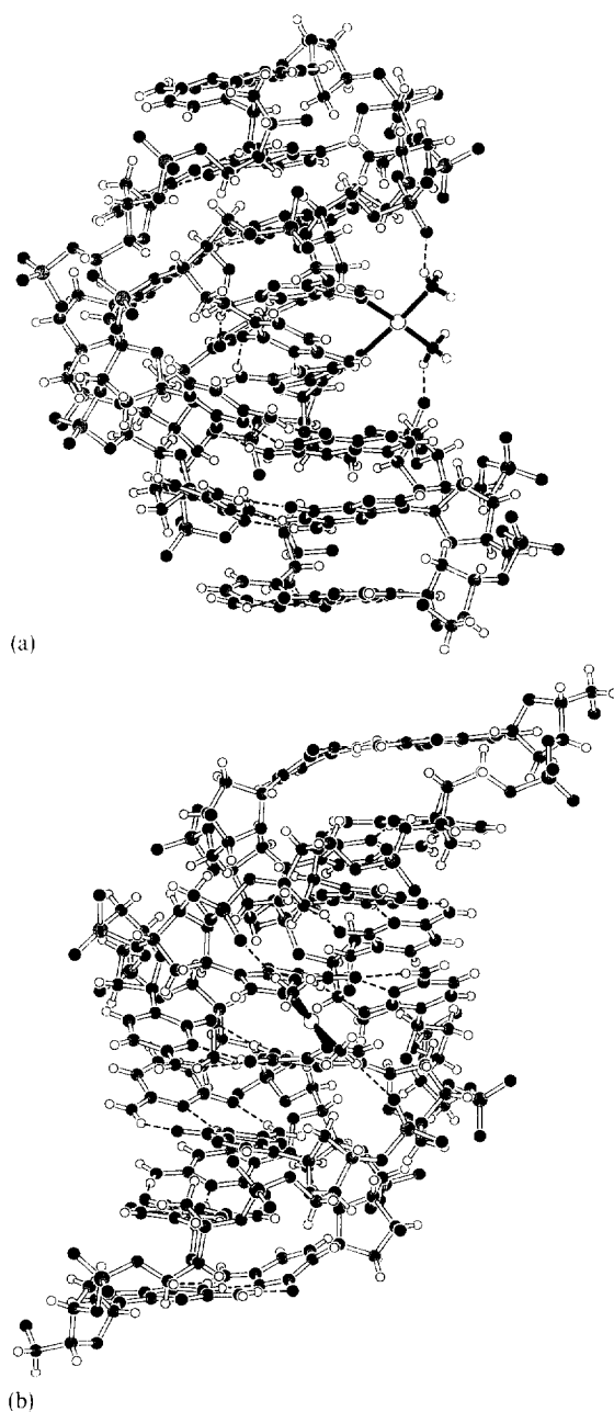
Fig. 6. Views along (a) and into (b) the major groove of a molecular mechanics model of the interstrand \text{Pt}(\text{NH}_3)_2 : (5'-d(GpGpGpG*pCpCpCpC)-3', 5'-d(GpGpGpG*pCpCpCpC)-3') adduct.
