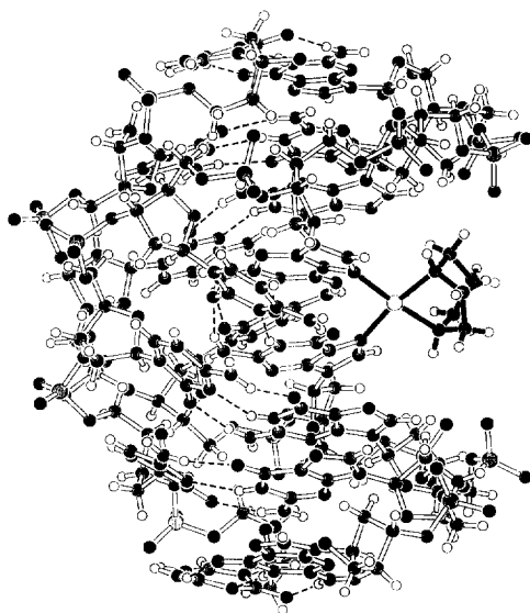
Fig. 8. Views along the major groove of a molecular mechanics model of the interstrand \text{Pt}(\text{hpic}) : (5'-d(GpGpGpG*pCpCpCpC)-3'; 5'-d(GpGpGpG*pCpCpCpC)-3') adduct.
