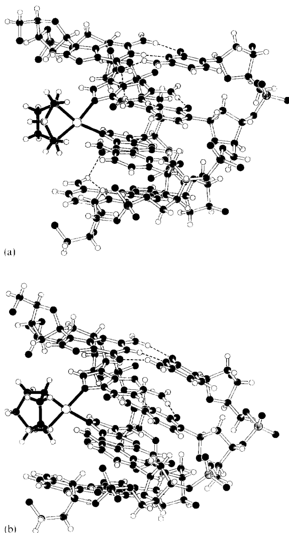
Fig. 12. Views of the molecular mechanics models of the isomers of the intrastrand adducts formed between \text{Pt}(\text{hpi})^{2+} and (5'\text{-d}(\text{GpGpGpG}^*\text{pG}^*\text{pGpGpG})\text{-3'}, 5'\text{-d}(\text{CpCpCpCpCpCpCpC})\text{-3'}) .
