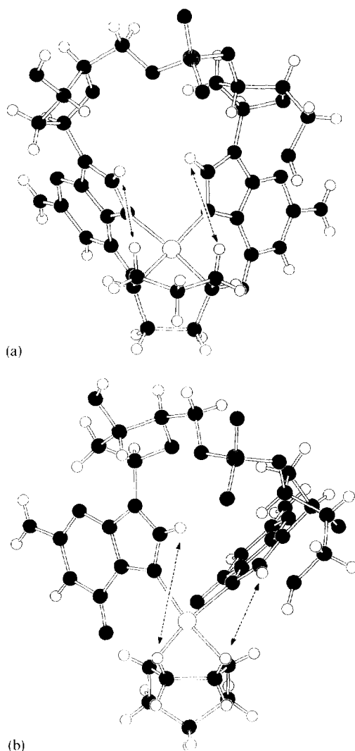
Fig. 11. Close contacts used to identify the isomers of [\text{Pt}(\text{hpip})(\text{GpG})] by NOESY correlations.
