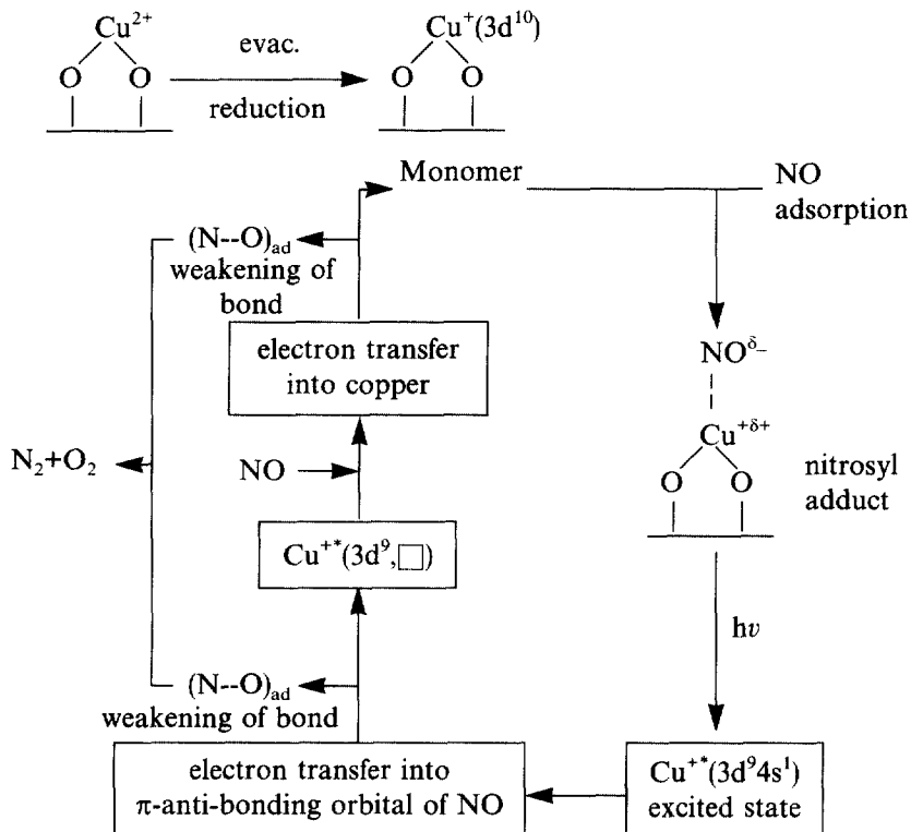
Scheme 1. Reaction scheme of the photocatalytic decomposition of NO into N 2 and O 2 on the Cu + /zeolite catalyst at 275 K.
