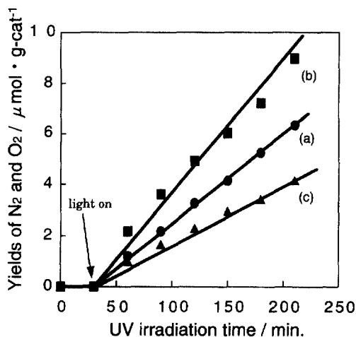
Fig. 6. Reaction profiles of the photocatalytic decomposition of N 2 O into N 2 and O 2 at 275 K on the Cu + /Y-zeolite catalysts with different Si/Al ratios: (a) 5.6, (b) 13.9, (c) 390.
