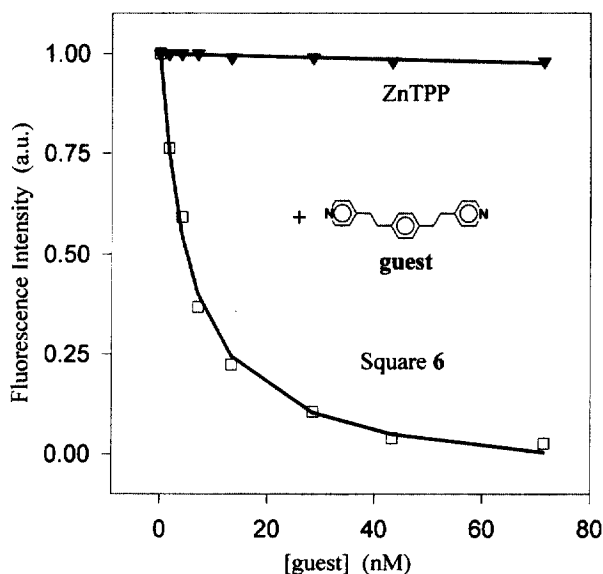
Fig. 7. Fluorescence intensity (at \lambda_{\text{em}} = 595 \text{ nm} ) of 6 ( \square ) and ZnTPP ( \nabla ) (both at 10^{-9} \text{ M} in CH 2 Cl 2 ) with addition of dipyriddy ligand guest. Solid lines correspond to the binding curve fits for ZnTPP and square 6.
