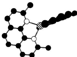
\text{Cu}(\text{dmp})_2^+
