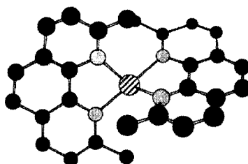
\text{Cu}(\text{dmp})_2^{2+}
