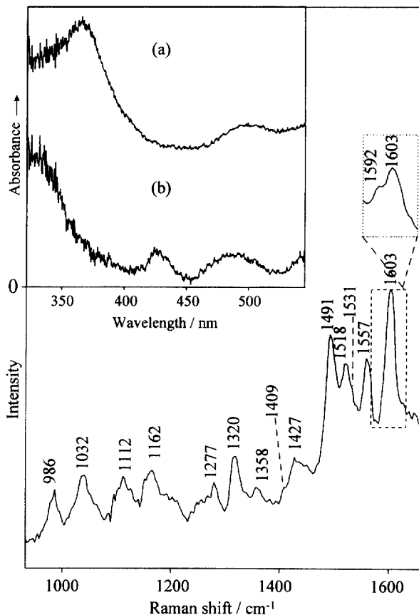
Fig. 1. Excited state RR spectra at \lambda_{\text{ex}}=355 nm using the single-colour pulse technique (laser pulse duration ca. 8 ns) of [(\text{Ru}(\text{bpy})_2\text{bpzt})]^{3+} in water; inset shows excited state absorption spectra recorded with \lambda_{\text{ex}}=416 nm of (a) [\text{Ru}(\text{bpy})_2\text{bpzt}]^+ and (b) [(\text{Ru}(\text{bpy})_2)_2\text{bpzt}]^{3+} , recorded using a gated multichannel diode array, 20 ns after laser excitation; the absorbance scale (arbitrary units) has been corrected for ground state depletion.
