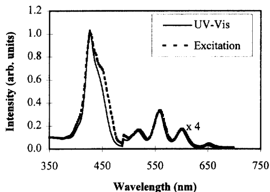
Fig. 8. Excitation spectrum of ZnFbPPP3 (monitored at 724 nm) compared with UV-vis spectrum of ZnFbPPP3 .
