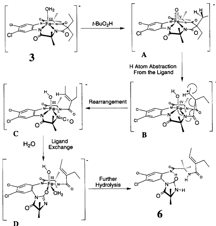
Scheme 2. Proposed ligand oxidative degradation scheme. In the scheme, we have drawn an \text{Fe}^{\text{V}} -oxo intermediate, A. With this, we do not wish to imply any specific allocation of oxidizing equivalents to the metal or the ligand. Alternative formulations include an \text{Fe}^{\text{IV}} -oxo/ligand radical cation. In addition, the abstracting entity could be a free radical.
