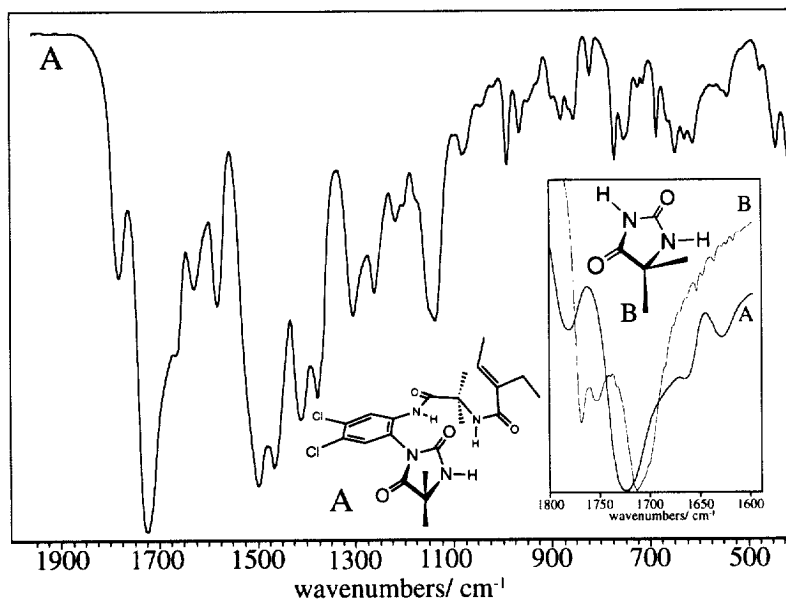
Fig. 11. The IR spectrum of solid 6 showing the strong 1723\text{ cm}^{-1} band. Insert: comparison of the 1600\text{--}1800\text{ cm}^{-1} region of 6 [A] and the parent dimethylhydantoin heterocycle [B].
