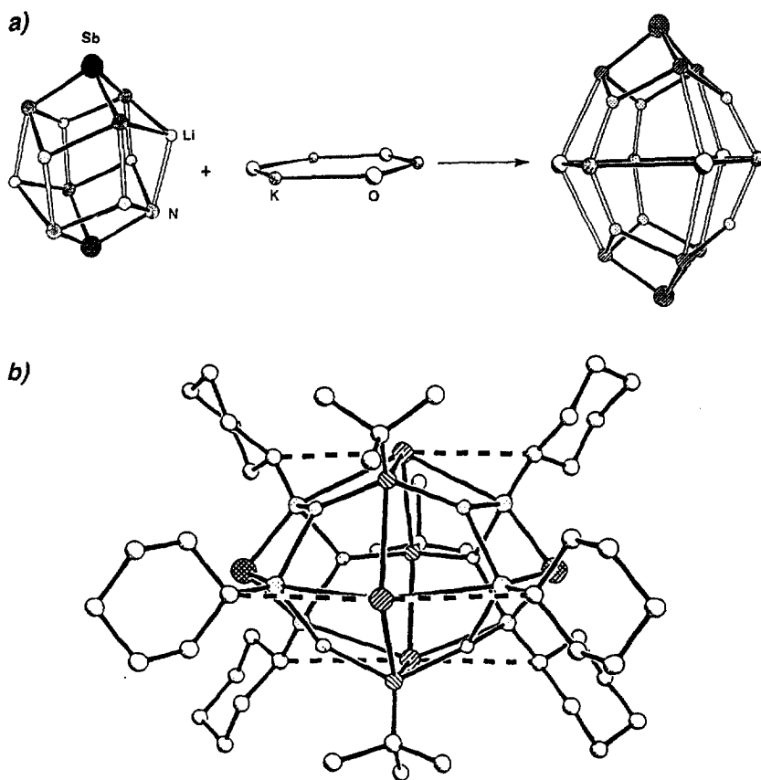
Fig. 12. (a) Schematic representation of the cage expansion of \{[\text{Sb}(\text{NCy})_3]_2\text{Li}_6 \cdot 2\text{HNMe}_2\} ( 9 ) with [\text{KOBu}'] and (b) structure of 12 .
