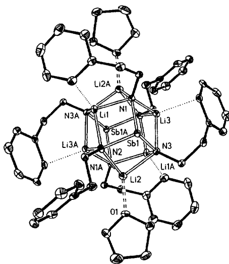
Fig. 6. The crystal structure of \{[\text{Sb}(\text{NCH}_2\text{CH}_2\text{Ph})_3]_2\text{Li}_6 \cdot \text{THF}\}_2 ( 6 ).
