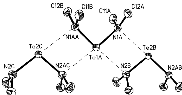
Fig. 26. The crystal structure of [\text{Te}(\text{NMe}_2)_2]_n (35).
