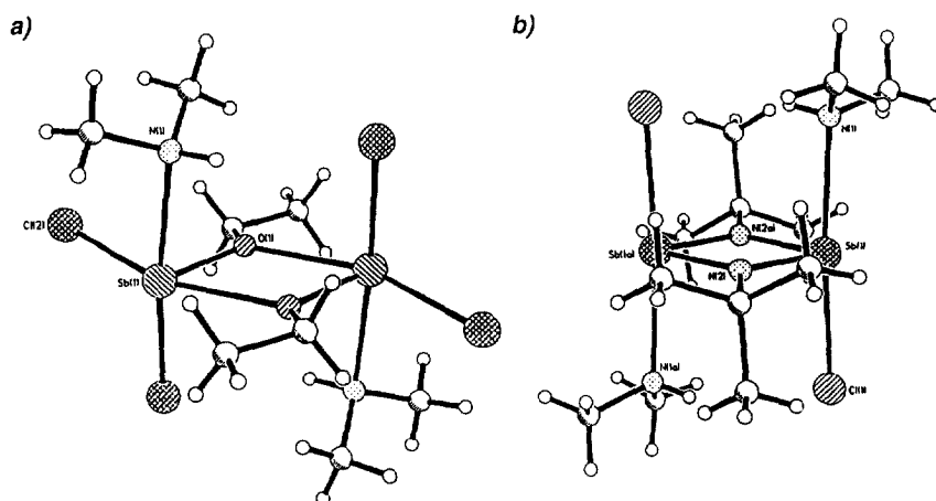
Fig. 3. The crystal structures of (a) [\text{SbCl}_2(\text{Me}_2\text{NH})(\mu\text{-OEt})_2]_2 (4) and (b) [\text{SbCl}(\text{Me}_2\text{NH})(\mu\text{-N}^t\text{Bu})]_2 (2).
