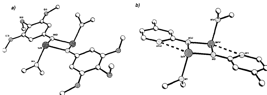
Fig. 1. The crystal structures of (a) \{\text{Me}_2\text{NSb}[\mu\text{-N(4-methylpyridin-2-yl)}]\}_2 (1) and (b) \{\text{Me}_2\text{NSb}[\mu\text{-NC}_6\text{H}_2(\text{OMe})_3\text{-3,4,5}]\}_2 (2).
