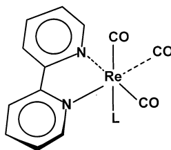
Fig. 15. Structure of (bpy)(phosphin)rheniumtricarboxyl complexes acting as photocatalyst in the photochemical CO 2 reduction [88–91].
