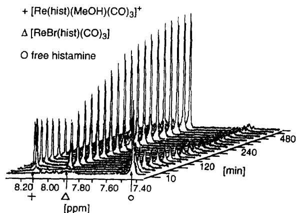
Fig. 5. Formation of [\text{ReBr}(\text{hist})(\text{CO})_3] ( 1b , [\text{hist}] = 27 mM) in d^4 -methanol at r.t. observed by ^1\text{H} NMR spectroscopy as a function of time.
