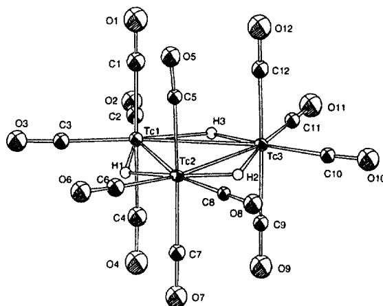
Fig. 1. ORTEP presentation of the mixed hydrido-carbonyl complex [\text{}^{99}\text{Tc}(\mu\text{-H})_3(\text{CO})_4]^{3-} .
