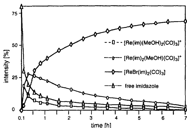
Fig. 4. Product distribution of the formation of imidazole complexes 3a , 4a and 4 as a function of time in d^4 -methanol at r.t., ( [\mathbf{1b}] = 30 \text{ mM} ) followed by ^1\text{H} NMR spectroscopy.
