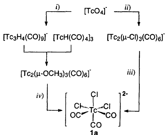
Scheme 2. Low pressure carbonylation of [^{99m}TcO_4]^- , in general: r.t., 1 atm CO, THF·BH 3 : (i) no Cl - ; (ii) with Cl - ; (iii) excess Cl - ; and (iv) NaOH in CH 3 OH then HCl.
