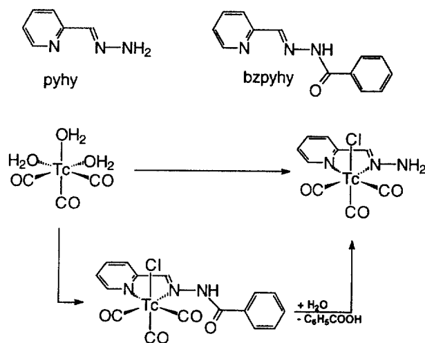
Scheme 7. Structure of pyhy and bzpyhy, synthesis of [\text{TcX}(\text{pyhy})(\text{CO})_3] , synthesis of [\text{TcX}(\text{bzpyhy})(\text{CO})_3] and subsequent hydrolysis at mild conditions.
