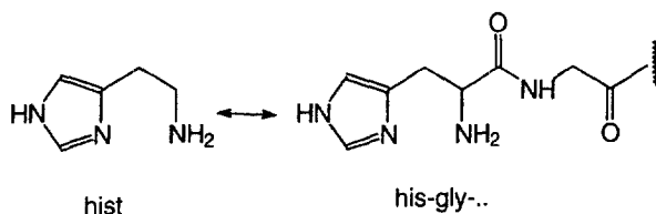
Scheme 5. Histamine mimics an N-terminal histidine in a peptide sequence.
