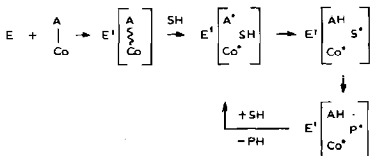
Scheme 2: Simplified description of \text{B}_{12} -dependent catalysis. E = apoenzyme; Co-A = coenzyme \text{B}_{12} ; \text{E}' [ ] = conformationally changed enzyme and its active site pocket; Co — A = conformationally changed coenzyme with a weakened Co-C bond; \text{Co}^\bullet = \text{B}_{12}\text{r} ; \text{A}^\bullet = 5' -deoxyadenosine radical, enzyme bound; \text{S}^\bullet and \text{P}^\bullet are substrate and product radicals.
