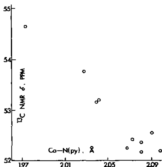
Fig. 15. ^{13}\text{C} NMR chemical shift of the \text{P}(\text{OMe})_3 group for \text{P}(\text{OMe})_3\text{Co}(\text{DH})_2\text{X} (Table 27) versus \text{Co}-\text{N}(\text{py}) distance for \text{pyCo}(\text{DH})_2\text{X} (Table 12). \text{X} = (top to bottom) \text{N}_3 ; \text{CH}_2\text{NO}_2 ; \text{CH}_2\text{CF}_3 ; \text{CH}_2\text{COOMe} ; \text{CH}_2\text{SiMe}_3 ; \text{CH}=\text{CH}_2 ; \text{CH}_2\text{CMe}_3 ; \text{Me} ; i\text{-C}_3\text{H}_7 ; \text{CH}_2\text{CH}_3 .
