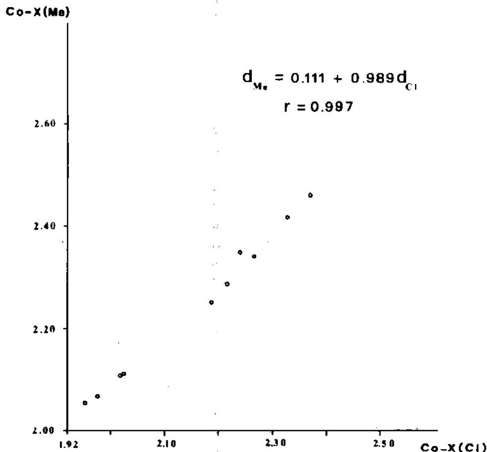
Fig. 8. Co-X ( X = O, N , and P) bond lengths trans to Me (a strong trans -influence ligand) against the corresponding bond lengths trans to Cl (a weak trans -influence ligand).
