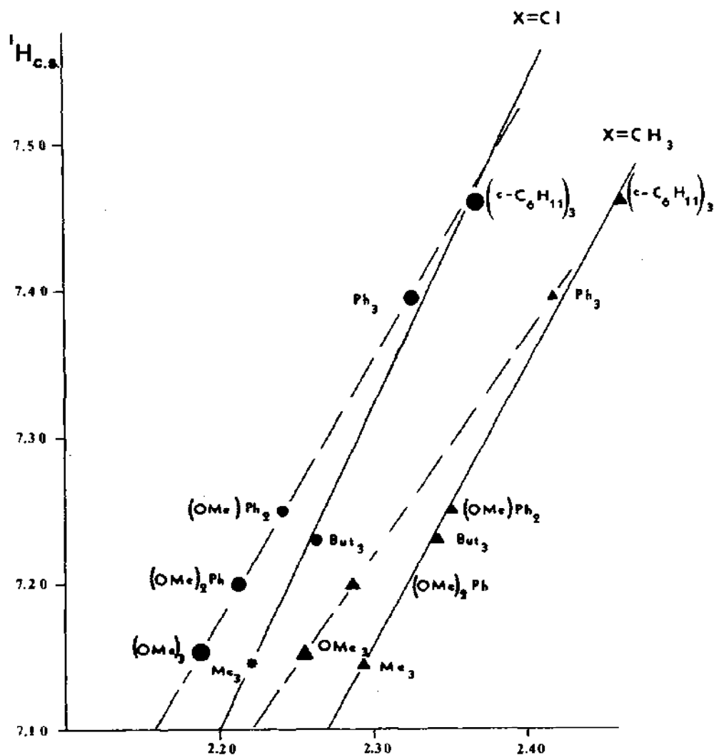
Fig. 12. ^1H NMR chemical shift of the Me group of methanol in [PR_3Co(DH)_2O(H)Me]^+ cations (Table 24) against Co-P bond lengths in PR_3Co(DH)_2X with X = Cl, Me (Table 11). Circles refer to X = Cl and triangles to X = Me .
