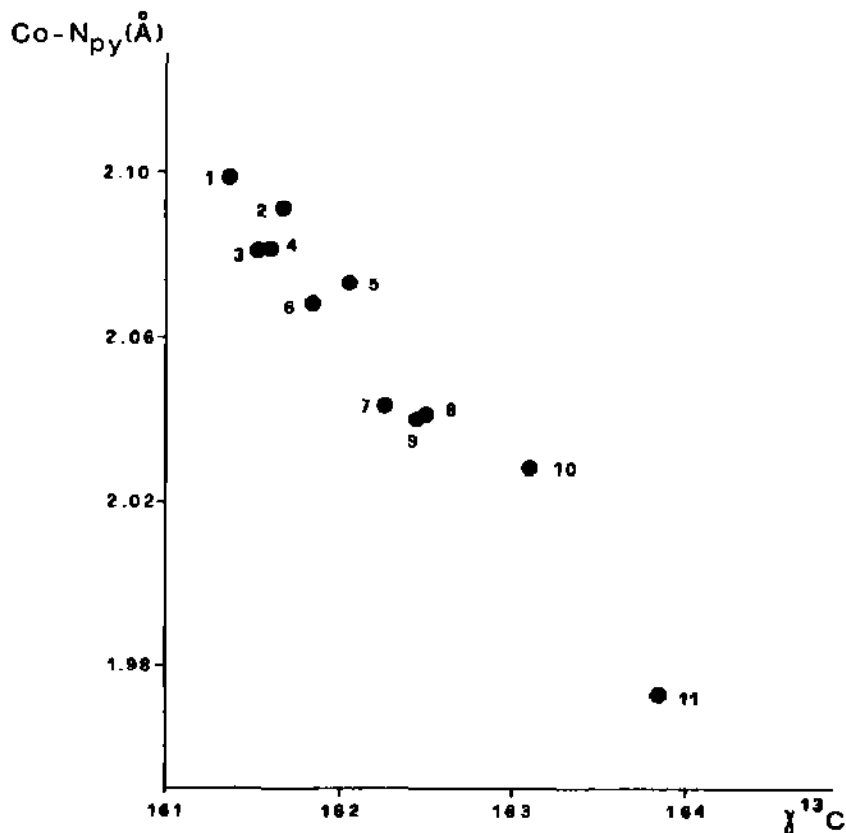
Fig. 14. Linear relationship between the Co-N(py) bond lengths in \text{pyCo}(\text{DH})_2\text{X} complexes and the \gamma\text{-}^{13}\text{C} chemical shift of 4-tBut-py analogues. 1 = i\text{-C}_3\text{H}_7 ; 2 = \text{CH}_2\text{SiMe}_3 ; 3 = \text{CH}_2\text{CMe}_3 ; 4 = \text{CH}_2\text{CH}_3 ; 5 = Me; 6 = \text{CH}=\text{CH}_2 ; 7 = \text{C}(\text{Cl})=\text{C}(\text{C}_6\text{H}_4\text{-}p\text{-Cl})_2 ; 8 = \text{CH}_2\text{COOMe} ; 9 = \text{CH}_2\text{CF}_3 ; 10 = \text{CH}_2\text{NO}_2 ; 11 = \text{N}_3 .
