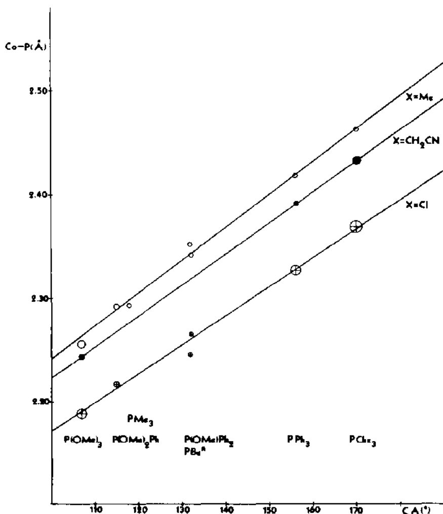
Fig. 6. Co-P distances against Tolman's cone angles in \text{PR}_3\text{Co}(\text{DH})_2\text{X} with \text{X} = \text{Cl}, \text{CH}_2\text{CN} , and Me (see ref. 71 for details).
