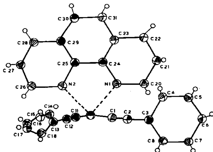
Fig. 3. ORTEP drawing of \text{Hg}(\text{Ph--C}\equiv\text{C})_2(\text{phen}) . The numbering of the hydrogen atoms (not shown) is that of the carbon atoms to which they are bonded. (Reproduced with permission from Acta Crystallogr., 34B (1978) 3382.)
