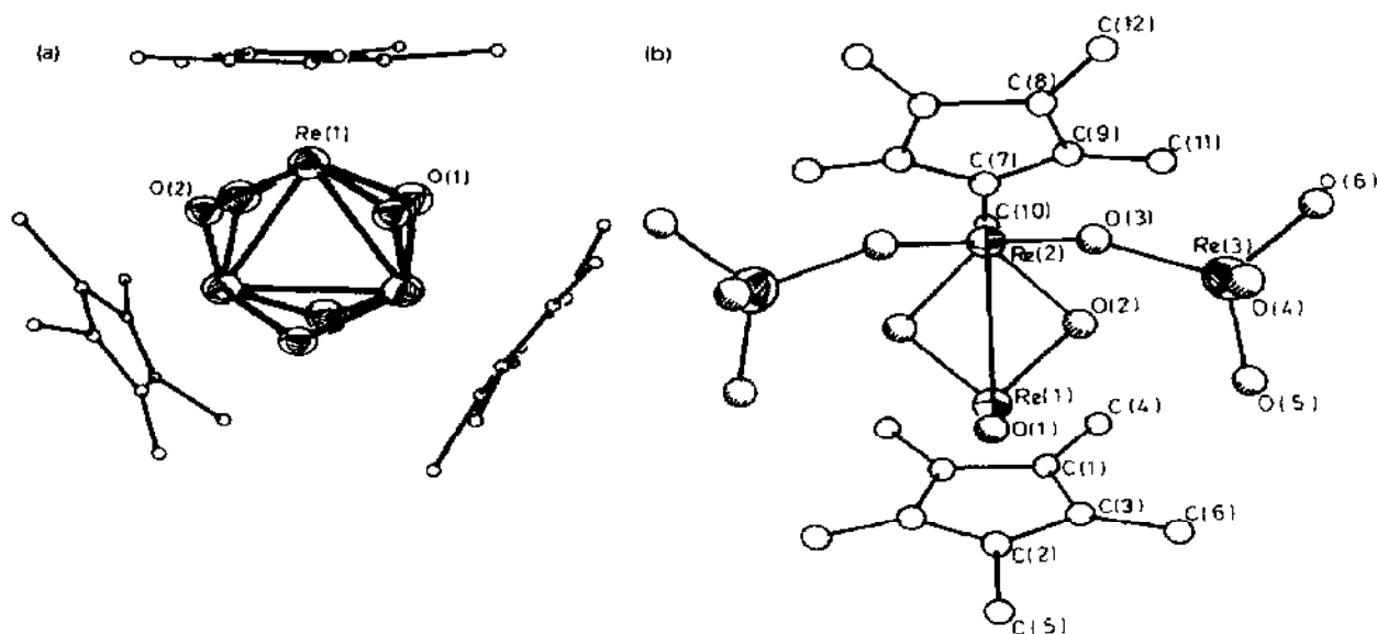
Fig. 65. Products from the reaction of \text{Cp}^*\text{ReO}_3 and \text{PPh}_3\text{-O}_2 . (a) Structure of the cation in [\text{Cp}_3^*\text{Re}_3\text{O}_6][\text{ReO}_4]_2 \cdot 0.5\text{CH}_2\text{Cl}_2 . Reproduced with permission from ref. 504. (b) Structure of \text{Cp}_2^*\text{Re}_4\text{O}_{11} . Reproduced with permission from ref. 506.
