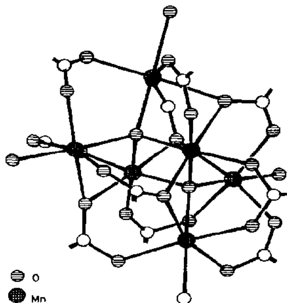
Fig. 54. The central core of the \text{Mn}_6\text{O}_2(\text{O}_2\text{C}^t\text{Bu})_{10}(\text{}^t\text{BuCO}_2\text{H})_4 cluster. The carboxylate ligands are only partially shown. Reproduced with permission from ref. 406.
