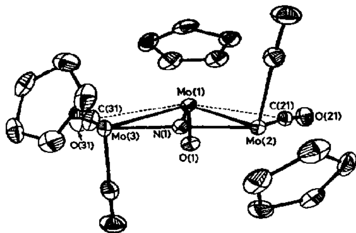
Fig. 30. Structure of Cp_3Mo_3(\mu_3-N)(O)(CO)_4 . Reproduced with permission from ref. 274.
