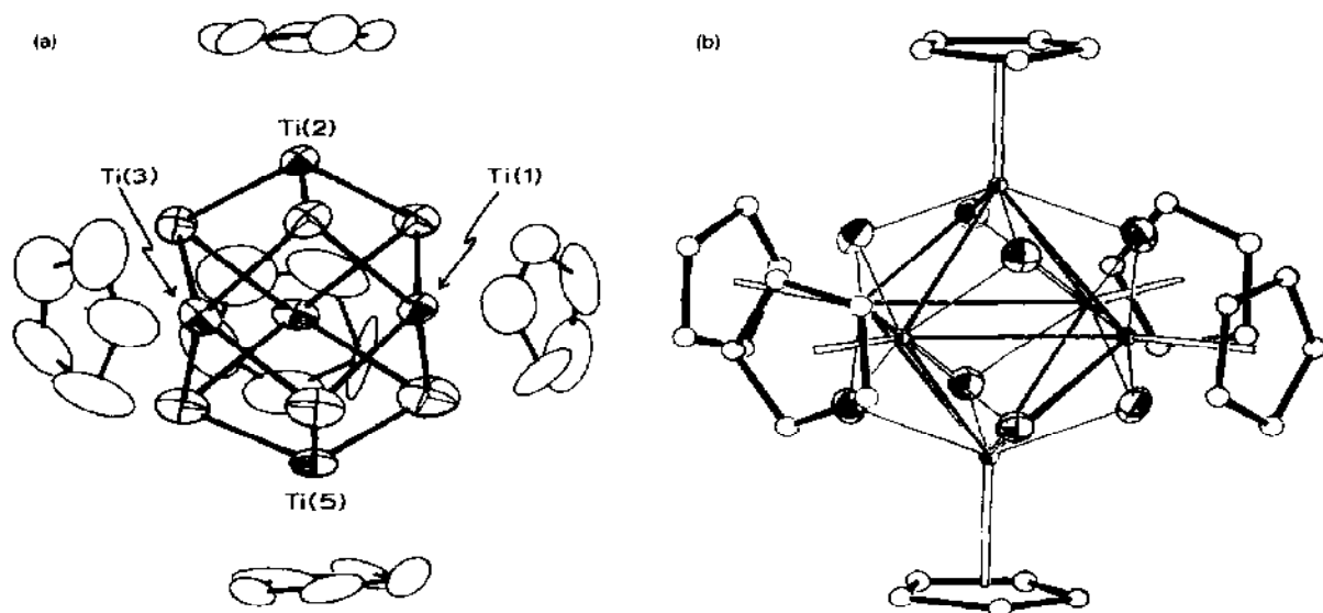
Fig 4. (a) The molecular structure of 12 . Average Ti-S distances are: Ti(1)-S = 2.474 \text{ \AA} , Ti(2)-S = 2.286 \text{ \AA} , Ti(3)-S = 2.463 \text{ \AA} , Ti(4)-S = 2.486 \text{ \AA} , Ti(5)-S = 2.272 \text{ \AA} . Reproduced with permission from ref. 33. (b) The structure of 13 at -160^\circ C . Titanium and oxygen atoms are shown as small and large sectioned atoms respectively, while carbon atoms are shown as open spheres. Reproduced with permission from ref. 34. The compounds 14 and 15 exhibit similar structures [37].
