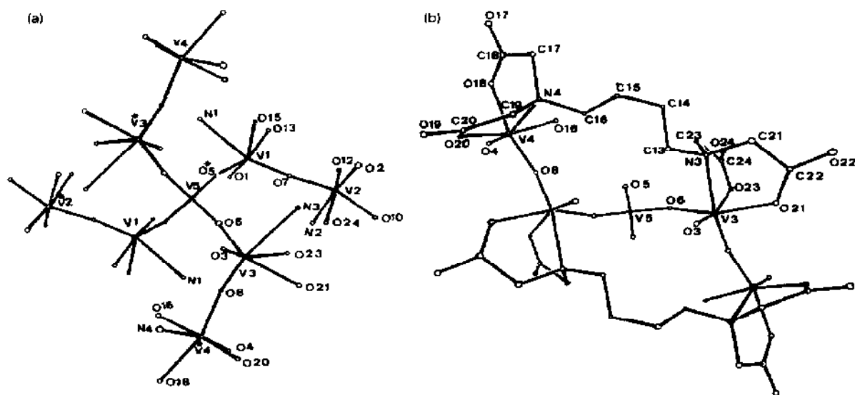
Fig. 11. Structure of the [V_9O_{16}(bdta)_4]^{7-} anion: (a) the arrangement of the V^{IV}V^V pairs about the central tetrahedral V^V atom; (b) the coordination mode of two of the bdta^{4-} ligands. Reproduced with permission from ref. 59.
