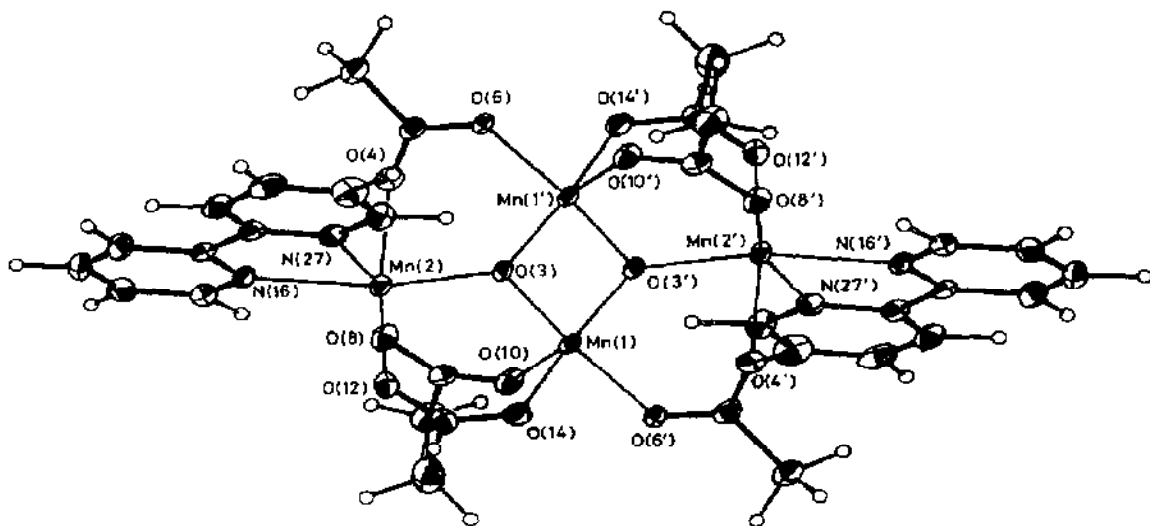
Fig. 53. Structure of 96 . Reproduced with permission from ref. 404.
