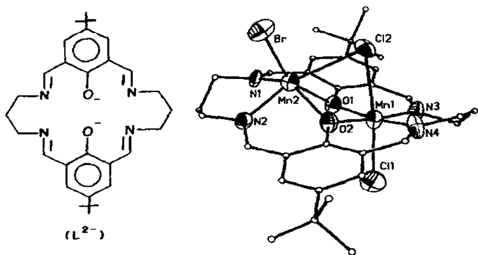
Fig. 47. Structure of \text{LMn}_2\text{Cl}_2\text{Br} where \text{L}^{2-} is the ligand shown. Reproduced with permission from ref. 386.
