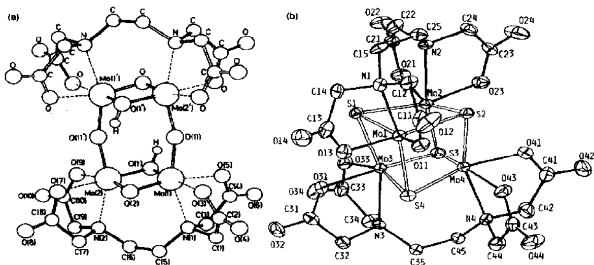
Fig. 34. (a) Structure of the anion in 61 . Reproduced with permission from ref. 283. (b) Structure of the anion in 63 . Reproduced with permission from ref. 285.
