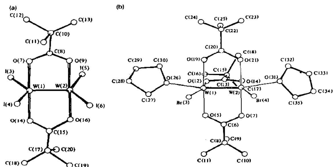
Fig. 41. (a) Structure of the [W_2I_4(O_2C'Bu)_2]^- anion in 76 . (b) Structure of W_2Br_2(O_2C'Bu)_3(thf)_2 . Reproduced with permission from ref. 327.
