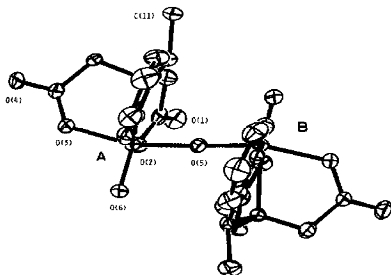
Fig. 7. Structure of the [V_2O_3(peida)_2]^- anion. Bond distances and angles include V_A-O(5) = 1.875(4) Å, V_B-O(5) = 1.763(4) Å, V_A-O(6) = 1.622(4) Å, V_B-O(6) = 1.613(4) Å, V_A-O(5)-V_B = 179.5(3)^\circ . Reproduced with permission from ref. 55.
