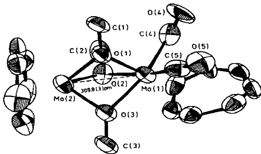
Fig. 27. The molecular structure of 48 . Reproduced with permission from ref. 247.
