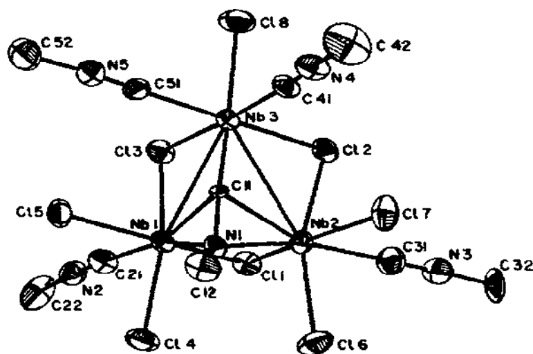
Fig. 15. The molecular structure of 28 drawn for clarity without the methyl groups of the t -BuNC ligands. Reproduced with permission from ref. 125.
