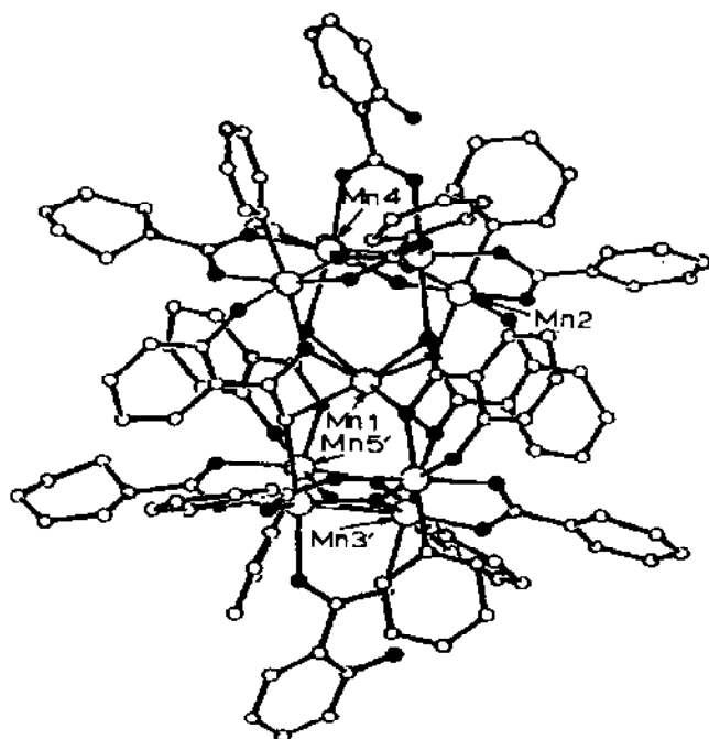
Fig. 55. Structure of \text{Mn}_9\text{O}_4(\text{O}_2\text{CPh})_8(\text{sal})_4(\text{salH})_2(\text{py})_4 with only one of each symmetry (C2) related pair of manganese atoms labelled. The oxygen atoms are shown as solid circles. Reproduced with permission from ref. 411.
