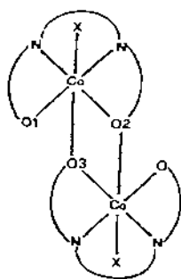
Fig. 2. A sketch of dimeric Co(salen) compounds.
