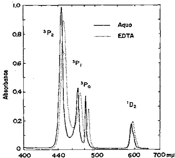
Fig. 1. Absorption Spectra of Aquo and EDTA Complexes of \text{Pr}^{\text{III}} in Aqueous Solutions.
