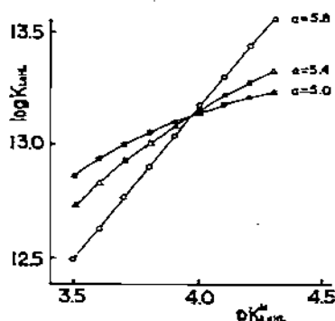
Fig. 5. Graphical solution for K_{LaHL} and K_{LaHL}^H (La: TPHA (1:1)).
