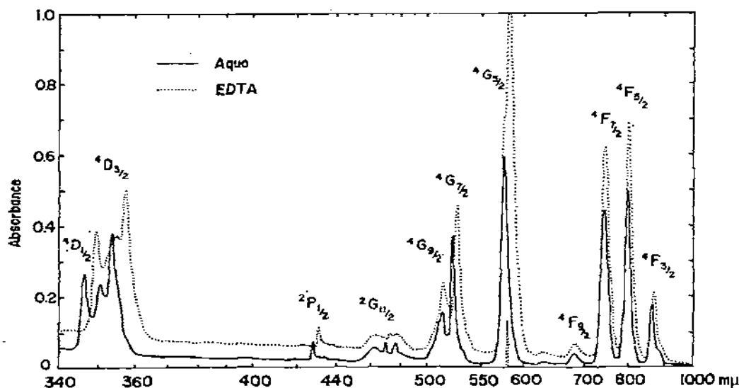
Fig. 2. Absorption Spectra of Aquo and EDTA Complexes of \text{Nd}^{\text{III}} in Aqueous Solutions.
