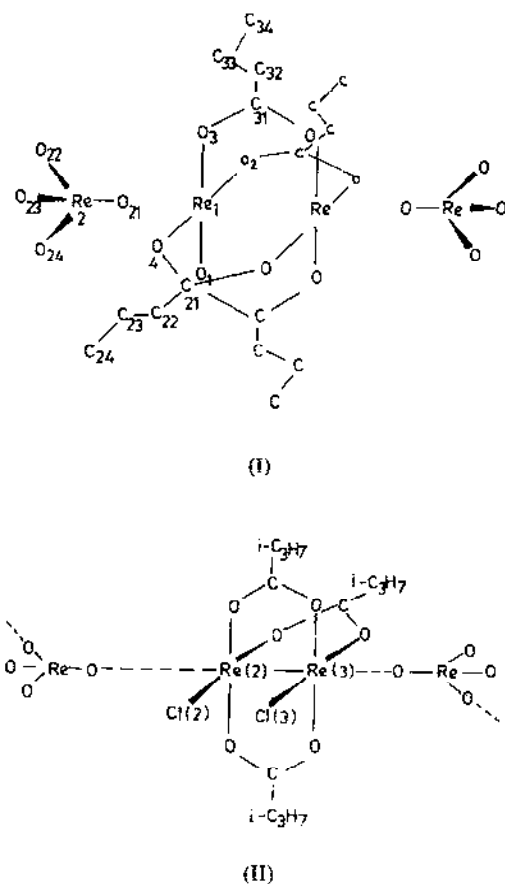
Fig. 4. Structures of [\text{Re}_2\text{Cl}_2(\text{iso-C}_3\text{H}_7\text{COO})_3](\text{ReO}_4) and [\text{Re}_2(n\text{-C}_3\text{H}_7\text{COO})_4](\text{ReO}_4)_2 . (Redrawn with permission from refs. 48 and 49.)
