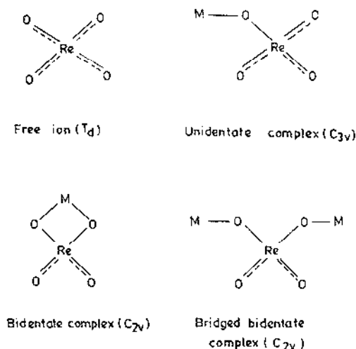
Fig. 1. Mode of coordination of [\text{ReO}_4]^- .
