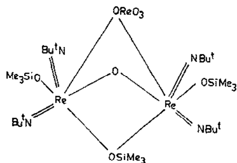
Fig. 5. Structure of \text{Re}_3(\text{N-}t\text{-Bu})_4\text{O}_5(\text{OSiMe}_3)_3 . (Redrawn with permission from ref. 58.)
