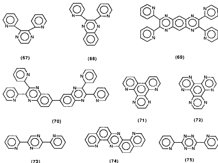
Fig. 9. Dipyriddyipyrazines and related ligands.
