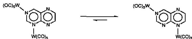
Fig. 2. Fluxional pteridine ditungsten complex.
