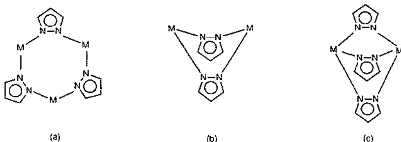
Fig. 4. Pyrazolate-bridged complexes.
