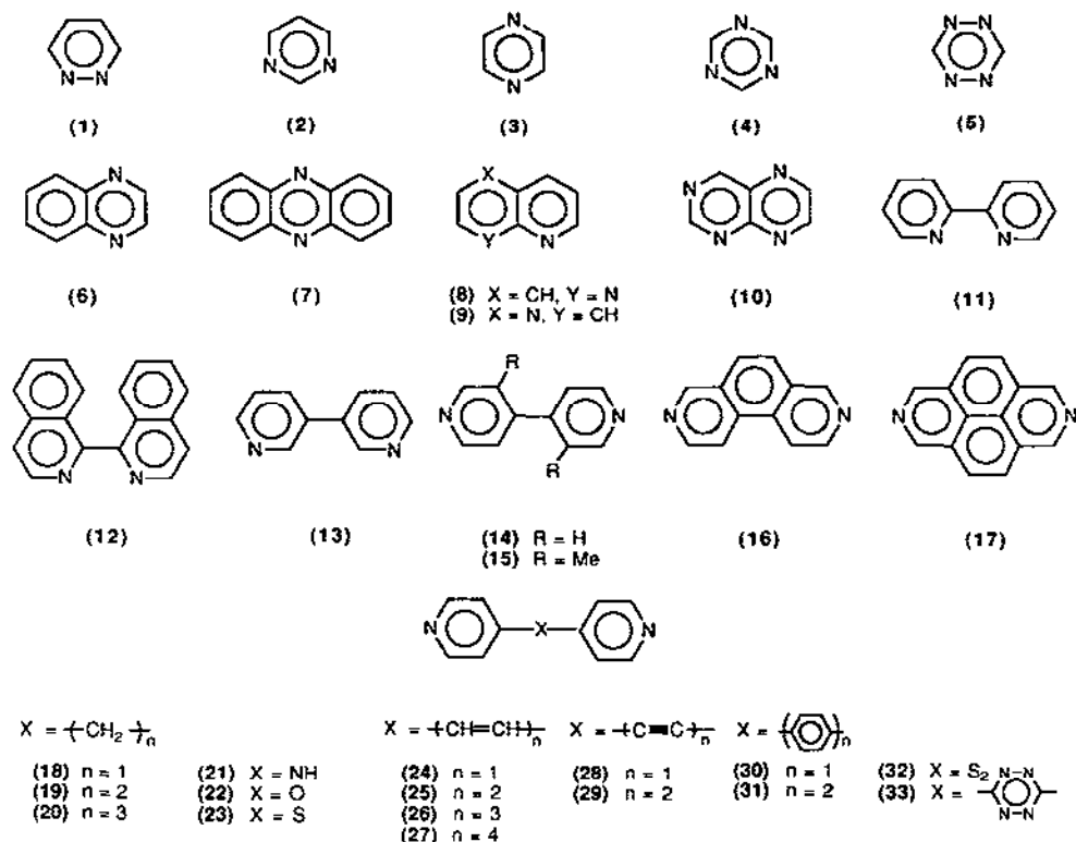
Fig. 1. Bridging azines.
