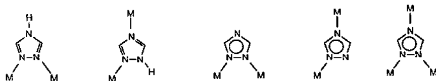
Fig. 5. Bridging modes of 1,2,4-triazole (38) and 1,2,4-triazolate (39).
