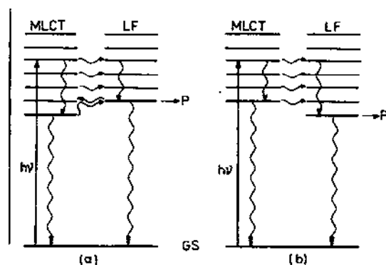
Fig. 15. Scheme of two extreme examples (a, b) of the "tuning model" for the photochemistry of [\text{Ru}(\text{NH}_3)_5(\text{py-X})]^{2+} complexes and analogous systems: (a) energetically lowest is the MLCT state (considerably reduced tendency for photosubstitution reaction), (b) energetically lowest is the LF state (increased tendency for photosubstitution reaction). P = products.
