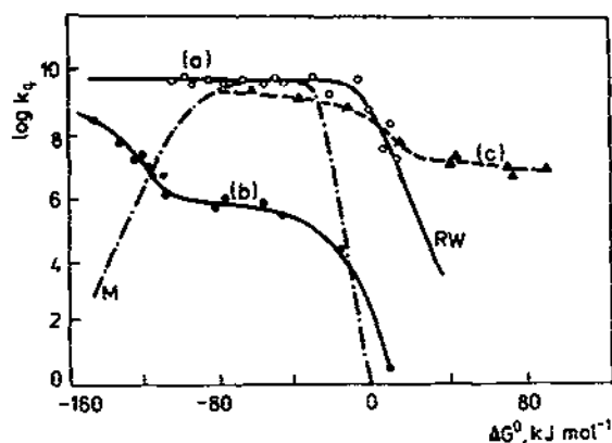
Fig. 10. Plots of \log k_q vs. \Delta G^0 for the following quenchings: (a) \circ — Redox quenching of [\text{Cr}(\text{bpy})_3]^{3+} by aromatic amines and methoxybenzenes [164]; curves RW and M represent the plots calculated according to the Rehm–Weller and Marcus relationships, respectively; (b) \bullet redox quenching of excited aromatics by aquated \text{Eu}^{2+} ions [151]; (c) \blacktriangle — redox and energy-transfer quenching of [\text{Cu}(\text{dpp})_2]^+ by aromatics and \text{Cr}(\text{III}) quenchers [175].
