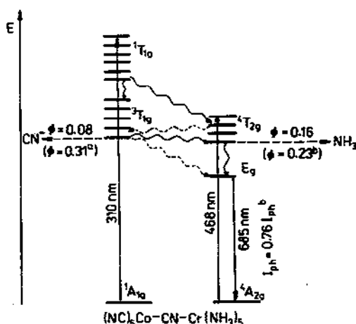
Fig. 6. Spectral properties and parameters of photophysical and photochemical deactivation processes of excited [(\text{NC})_5\text{Co-CN-Cr}(\text{NH}_3)_5]^* . a Corresponding values for [\text{Co}(\text{CN})_6]^{3-} complex. b Values for the binuclear complex in the ^4T_{2g} excited state; the other values are for the binuclear complex in its ^1T_{1g} excited state.
