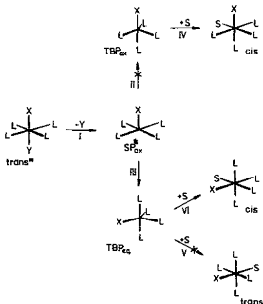
Fig. 19. Dissociative mechanism for ligand photosubstitution ( \text{S} \neq \text{Y} ) (VC model) and trans-cis photoisomerization ( \text{S} = \text{Y} ) in excited tetragonal d^3 \text{ML}_4\text{XY} complexes. \text{SP}_4^{\text{ax}} = excited square pyramidal \text{ML}_4\text{X} fragment, \text{TBP} = ground-state trigonal-bipyramidal intermediate with an axial X ligand ( \text{TBP}_{\text{ax}} ) or an equatorial X ligand ( \text{TBP}_{\text{eq}} ), S = solvent molecule, X = symmetry-forbidden paths.
