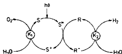
Fig. 27. System for photochemical reduction of \text{H}_2\text{O} to \text{H}_2 , \text{S} = [\text{Ru}(\text{bpy})_3]^{2+} , [\text{Zn}(\text{TMPy})]^{2+} ; \text{D} = \text{TEOA} , \text{EDTA} ; \text{R} = \text{MV}^{2+} , \text{Eu}^{3+} , \text{V}^{3+} and their salicylate complexes; [\text{Ru}(\text{bpy})_3]^{3+} , macrocyclic complexes of cobalt; \text{K}_2 = \text{colloidal Pt} , \text{TEOA} = \text{triethanolamine} ; \text{EDTA} = \text{ethylenediaminetetraacetic acid} ; \text{MV}^{2+} = \text{methylviologen} ; 4,4'-dimethylpyridine.
