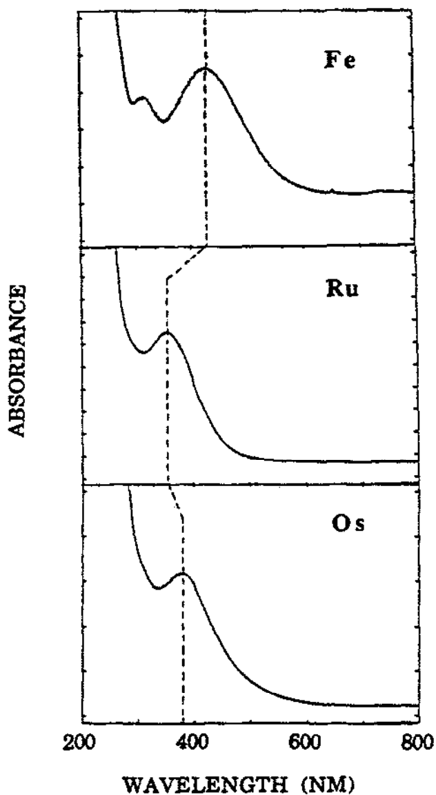
Figure 1. UV-vis absorption spectra for [\text{Pt}(\text{NH}_3)_4]_2^{4+} \{[(\text{NC})_5\text{M}^{\text{II}}\text{CN}-\text{Pt}^{\text{IV}}(\text{NH}_3)_4\text{NC-M}^{\text{II}}(\text{CN})_5]^{4-}\} , where \text{M}=\text{Fe} (top), \text{Ru} (middle), and \text{Os} (bottom).
