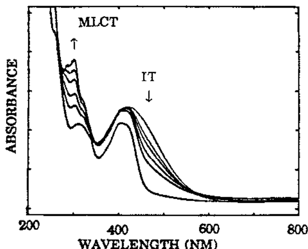
Figure 2. Electronic absorption spectra of \{[\text{Pt}(\text{NH}_3)_4]_2^{4+}\} \{[(\text{NC})_5\text{Fe-CN-Pt}(\text{NH}_3)_4\text{-NC-Fe}(\text{CN})_5]^{4-}\} in aqueous solution as a function of photolysis (488 nm) time. The arrows indicate the growth and decline of peaks with time.
