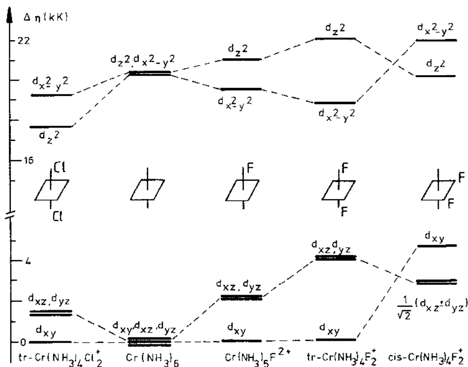
Figure 2. Relative orbital energies ( \eta ) in overall substituted chromium(III) amines [Taken from ref 14].
