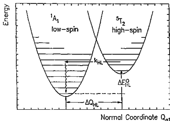
Fig. 2 : Potential wells for the HS and the LS state of Fe(II) in octahedral coordination along the totally symmetric normal coordinate.
