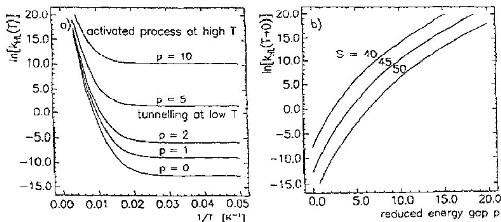
Fig. 9: a) \ln[k_{HL}(T)] vs. 1/T calculated with S = 45 and \hbar\omega = 250 \text{ cm}^{-1} and the reduced energy p as parameter. b) Calculated low T tunneling rate constants \ln[k_{HL}(T \rightarrow 0)] vs. p with \hbar\omega = 250 \text{ cm}^{-1} and S as parameter (from ref. [17]).
