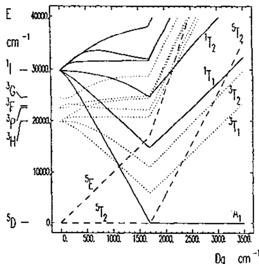
Fig. 1 : Tanabe-Sugano diagram for a d^6 -system.
