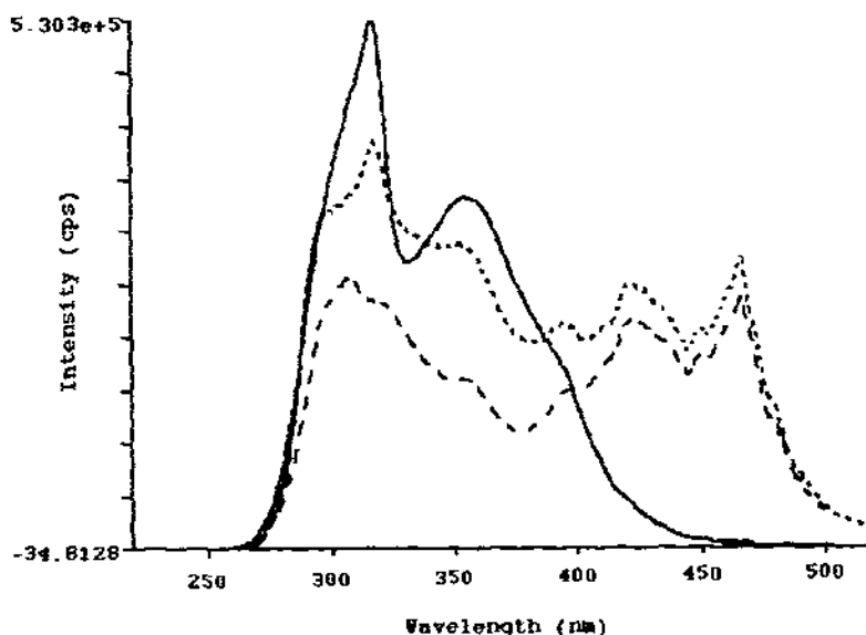
Figure 3. A comparison of the excitation spectra of [(bpy)_2Ru(Mebpy-Mebpy)]^{2+} (—), [(Mebpy-Mebpy)Re(CO)_3py]^+ (----), and [(bpy)_2Ru(Mebpy-Mebpy)Re(CO)_3py]^{3+} (.....). The [(bpy)_2Ru(Mebpy-Mebpy)Re(CO)_3py]^{3+} emission was monitored at 610 nm; the [(bpy)_2Ru(Mebpy-Mebpy)]^{2+} emission was monitored at 610 nm (its excitation spectrum was multiplied by 0.62); the [(Mebpy-Mebpy)Re(CO)_3py]^+ emission was monitored at 550 nm (its excitation spectrum was multiplied by 0.38).
