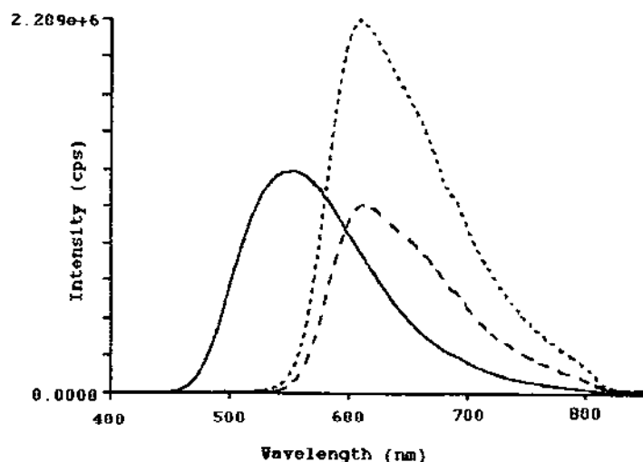
Figure 2. An emission spectral comparison of [(\text{Mebpy-Mebpy})\text{Re}(\text{CO})_3\text{py}]^{3+} (—), [(\text{bpy})_2\text{Ru}(\text{Mebpy-Mebpy})]^{2+} (----), and [(\text{bpy})_2\text{Ru}(\text{Mebpy-Mebpy})\text{Re}(\text{CO})_3\text{py}]^{3+} (.....) in \text{CH}_2\text{Cl}_2 ( \lambda_{\text{ex}} = 355 \text{ nm} ).
