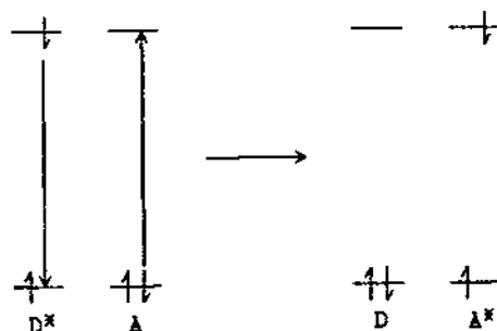
Scheme 3. The dipole-dipole interchange mechanism.
