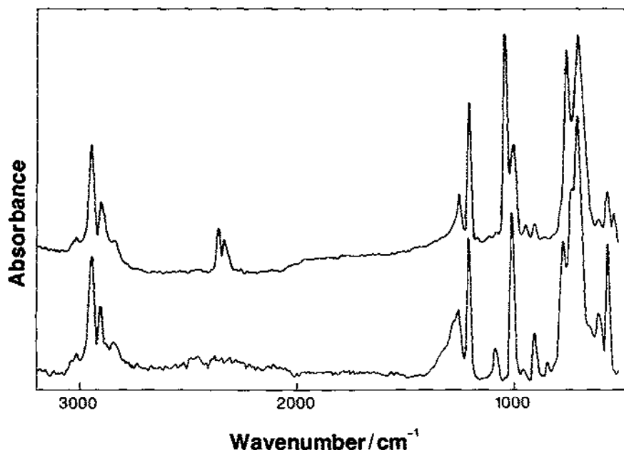
Fig. 8. As for Fig. 7 with DMAID in place of DMAIH. The new strong feature near 1040\text{ cm}^{-1} arises from \text{Me}_2\text{Al}(\mu\text{D})(\mu\text{Me})\text{AlMe}_2 ; the doublet near 2300\text{ cm}^{-1} in the top spectrum arises from \text{CO}_2 .
