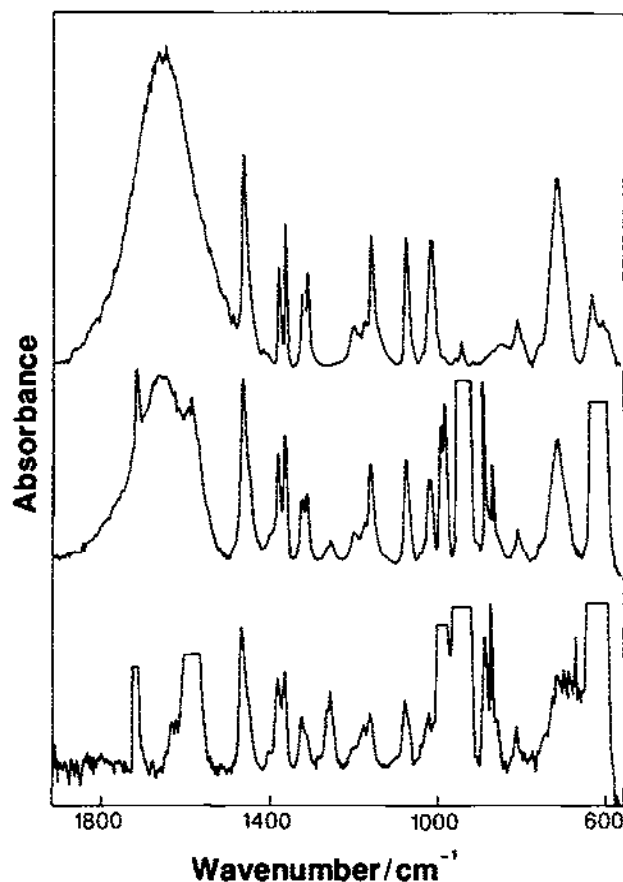
Fig. 19. As for Fig. 18 with TBGa in place of 1BGa. In this case, evidence for two Ga-H bending peaks is less clear.
