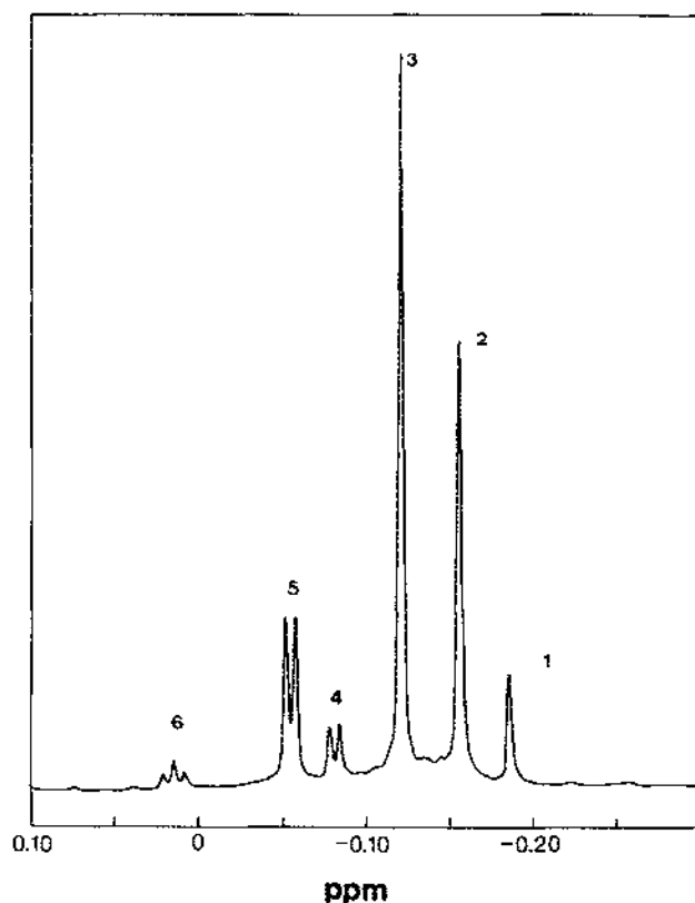
Fig. 22. ^1\text{H} NMR spectrum (300 MHz, 0.10 to -0.30 ppm, -60^\circ\text{C} ) of the product of IR LPHP of a 1:1 mixture of TMGa and TEGa on addition of \text{NMe}_3 in d_6 -toluene. Signals are assigned to methyl resonances in 1, \text{MeEt}_2\text{Ga}\cdot\text{NMe}_3 ; 2, \text{Me}_2\text{EtGa}\cdot\text{NMe}_3 ; 3, \text{Me}_3\text{Ga}\cdot\text{NMe}_3 ; 4, \text{MeEtGaH}\cdot\text{NMe}_3 ; 5, \text{Me}_2\text{GaH}\cdot\text{NMe}_3 ; and 6, \text{MeGaH}_2\cdot\text{NMe}_3 ; the doublets or triplets arise from coupling to Ga-H protons.
