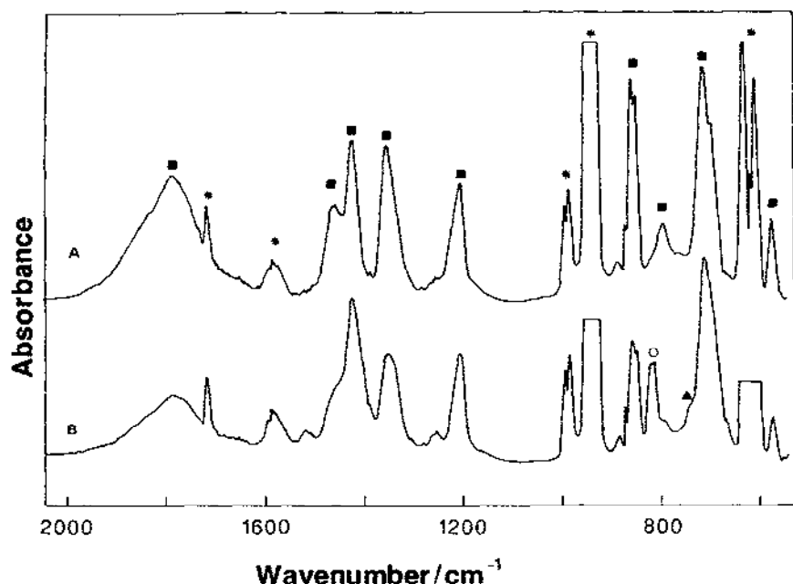
Fig. 5. FTIR spectra of a mixture of \text{SF}_6 (10 torr) and \text{DMAIH} (2 torr) before (top) and after (bottom) exposure to 5 W IR laser irradiation for 17 s. Features identified arise from \text{SF}_6 (★), \text{DMAIH} (■), and the \text{AlMe}_2 rocking (○) and \text{Al-F} stretching (▲) of the mixed bridged \text{Me}_2\text{Al}(\mu\text{H})(\mu\text{F})\text{AlMe}_2 .
