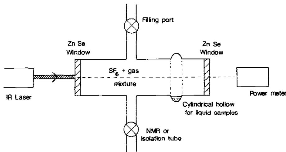
Fig. 2. Essentials of the IR LPHP technique. The ZnSe windows provide access for FTIR monitoring as well as for IR laser irradiation.
