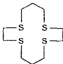
[14]aneS 4
