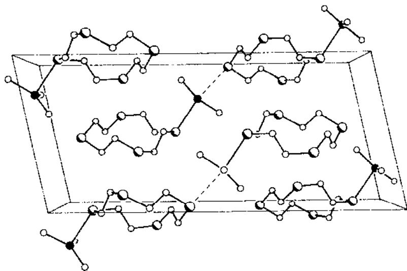
Fig. 5. Crystal packing diagram of [\text{12}] \text{aneS}_4[\text{Me}_3\text{Al}] viewed along the b axis. The broken line indicates a secondary interaction.
