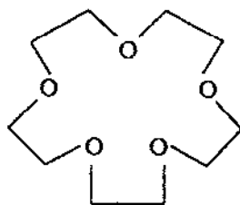
15-crown-5
