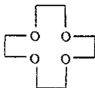
12-crown-4
