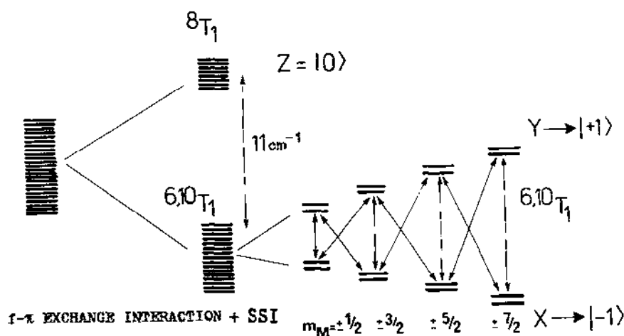
Fig. 9. Energy level diagram of \text{Gd}(\text{acac})_3(\text{bpy}) triplet state when the f-p\pi exchange interaction and SSI are taken into account. Arrows mark microwave transitions corresponding to the resonances shown in Fig. 8.
