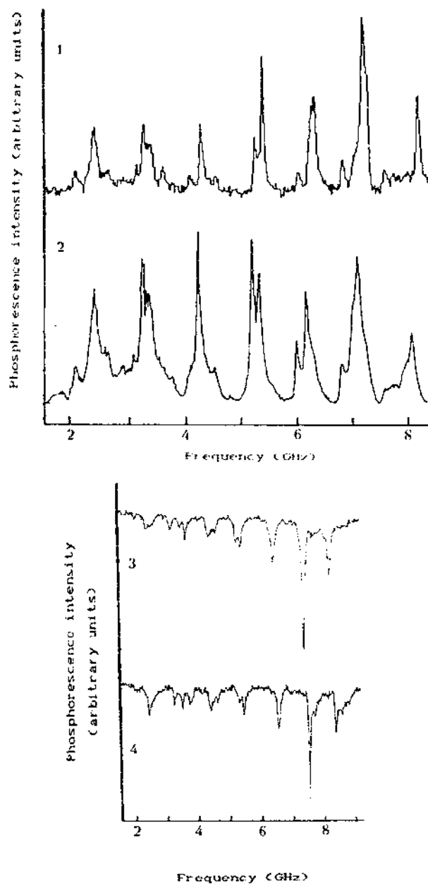
Fig. 8. PMDR signals of \text{Gd}(\text{acac})_3(\text{bpy}) (1), \text{Gd}(\text{NO}_3)_3(\text{bpy})_2 (2), \text{Gd}(\text{acac})_3(\text{phen}) (3) and \text{Gd}(\text{NO}_3)_3 \cdot (\text{phen})_2 (4) in crystal state at 5 K [138,152].
