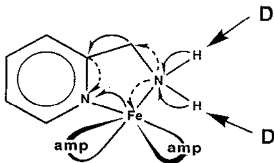
Fig. 10. Scheme of electron redistribution and bond length variation in \text{Fe}(\text{amp})_3(\text{B}\phi_4) induced by interaction of the amino protons with donor solvent molecules, D.
