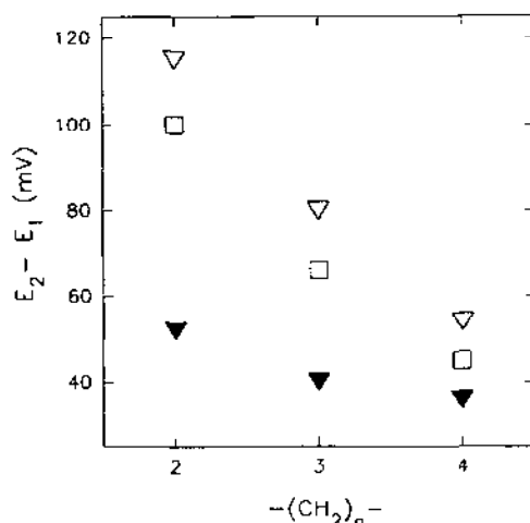
Fig. 4. Effect of the length of the connecting -(CH_2)_n- chain on the potential difference, \Delta E , for the second and first oxidation step of the homo-dimetallic complexes Ni_2^{II}(14-n-14-biscyclam)](ClO_4)_4 and [Cu_2^{II}(14-n-14-biscyclam)](ClO_4)_4 . □, Ni in MeCN; ▼, Ni in 70% HClO_4 ; ▽, Cu in 70% HClO_4 .
