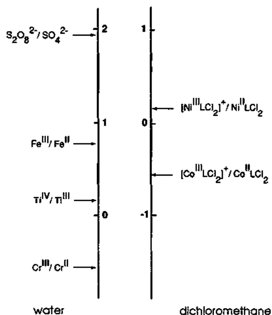
Fig. 9. Using a lipophilic metallocyclam complex to transport electrons across liquid membranes. Juxtaposition of the electrochemical scale in water (potentials vs. SHE) and of the electrochemical scale in the solvent used as liquid membrane, e.g. CH_2Cl_2 (potentials vs. the Fc^+/Fc internal reference; L is the lipophilic version of cyclam, 17). Changing of the metal (Co or Ni) allows the electron carrier system to be positioned in the cathodic or anodic part of the scale.
